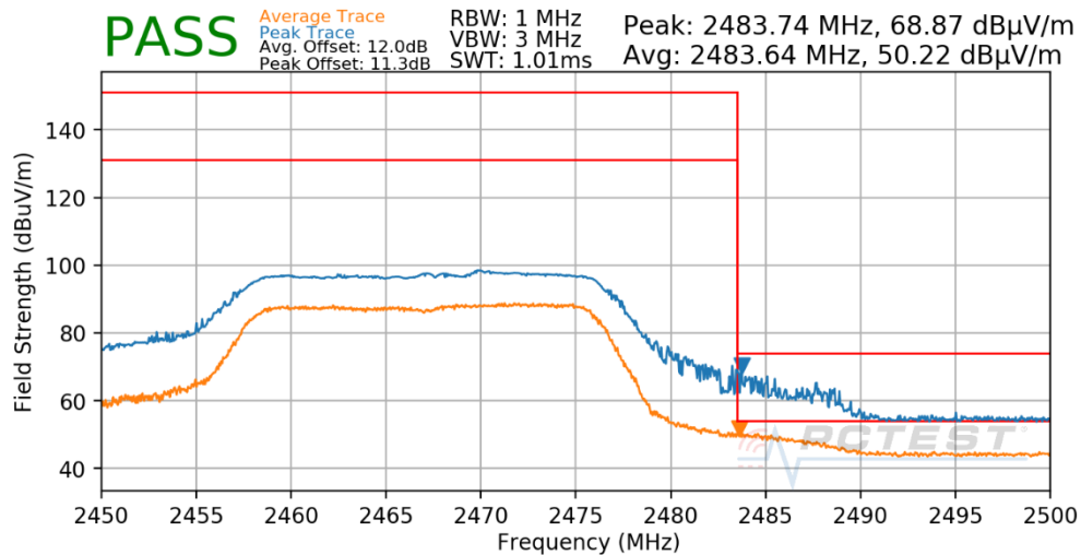
Plot 7-52. Radiated Restricted Upper Band Edge Measurement
