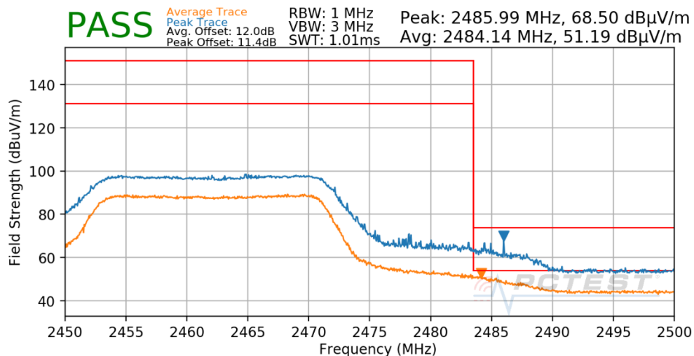
Plot 7-51. Radiated Restricted Upper Band Edge Measurement
