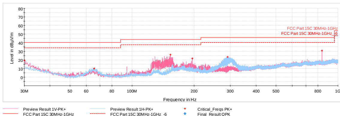
Plot 7-38. Radiated Spurious Emissions 30MHz-1GHz (1Mbps, ePA – Ch.39, with WCP + laptop)
