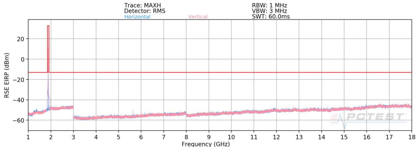
Plot 7-47. Radiated Spurious Emissions above 1GHz (PCS WCDMA Mode – Ch. 9400)
