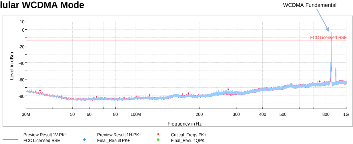
Plot 7-44. Radiated Spurious Emissions below 1GHz (Cellular WCDMA Mode – Ch. 4233)
