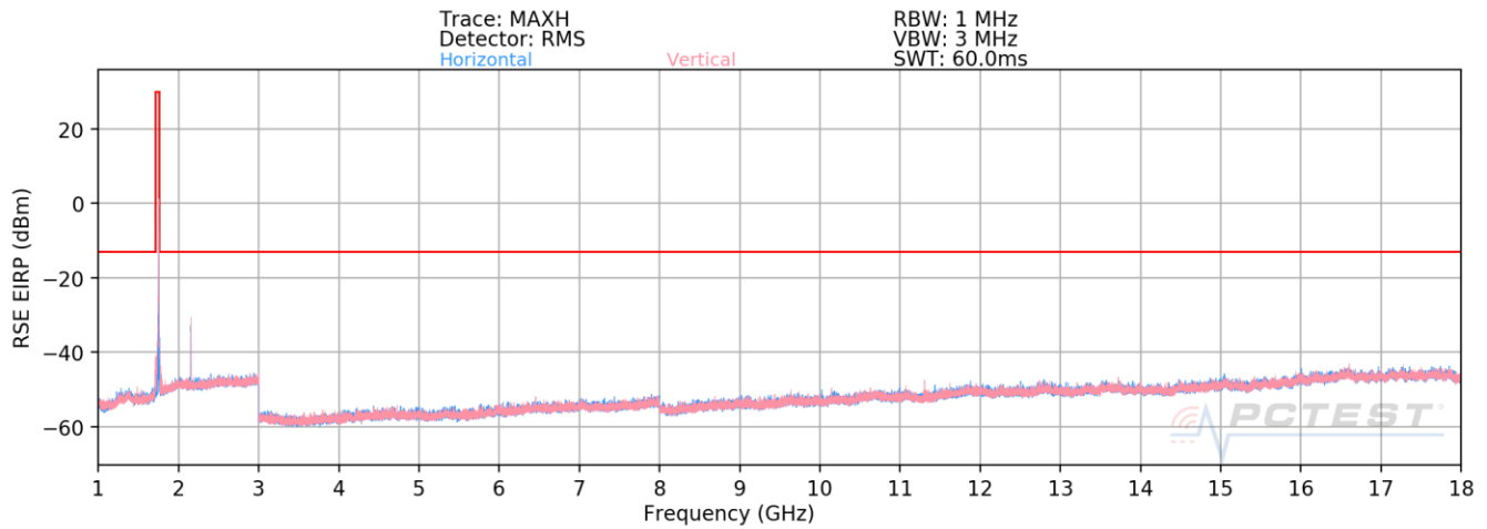
Plot 7-46. Radiated Spurious Emissions above 1GHz (AWS WCDMA Mode – Ch. 1513)
