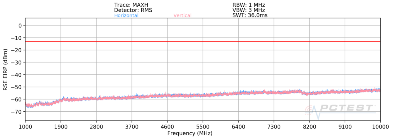
Plot 7-45. Radiated Spurious Emissions above 1GHz (Cellular WCDMA Mode – Ch. 4233)
