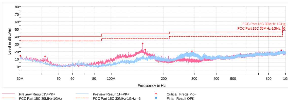
Plot 7-38. Radiated Spurious Emissions 30MHz-1GHz (1Mbps, ePA – Ch.19, with WCP + laptop)
