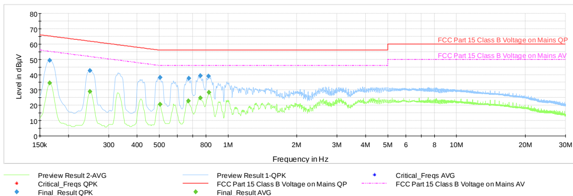
Plot 7-40. AC Line Conducted Emission Bluetooth LE (N - 1Mbps, ePA, Ch.19, with WCP + AC/DC Adapter)
