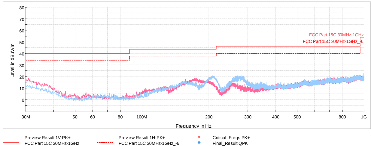
Plot 7-10. Radiated Spurious Emissions 30MHz – 1GHz (CE B 848kbps, with WCP + AC/DC Adapter)
