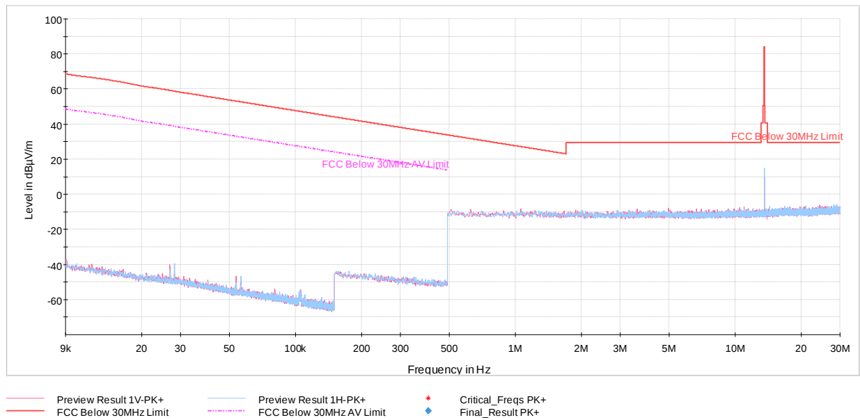
Plot 7-8. Radiated Spurious Emissions 9kHz – 30MHz (CE B 848kbps, with WCP + AC/DC Adapter)
