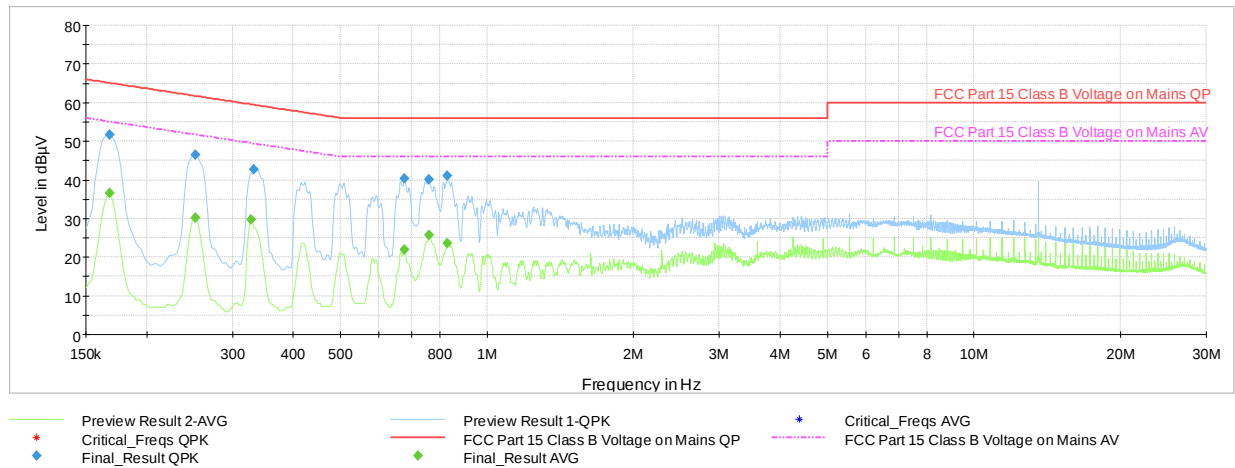
Plot 7-12. AC Line-Conducted Test Plot (L1, CE B 848kbps, with WCP + AC/DC Adapter)
