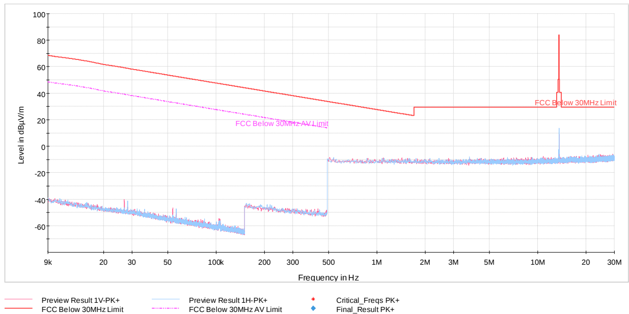
Plot 7-9. Radiated Spurious Emissions 9kHz – 30MHz (Reader 10% Ask 1 out of 4, with WCP + AC/DC Adapter)
