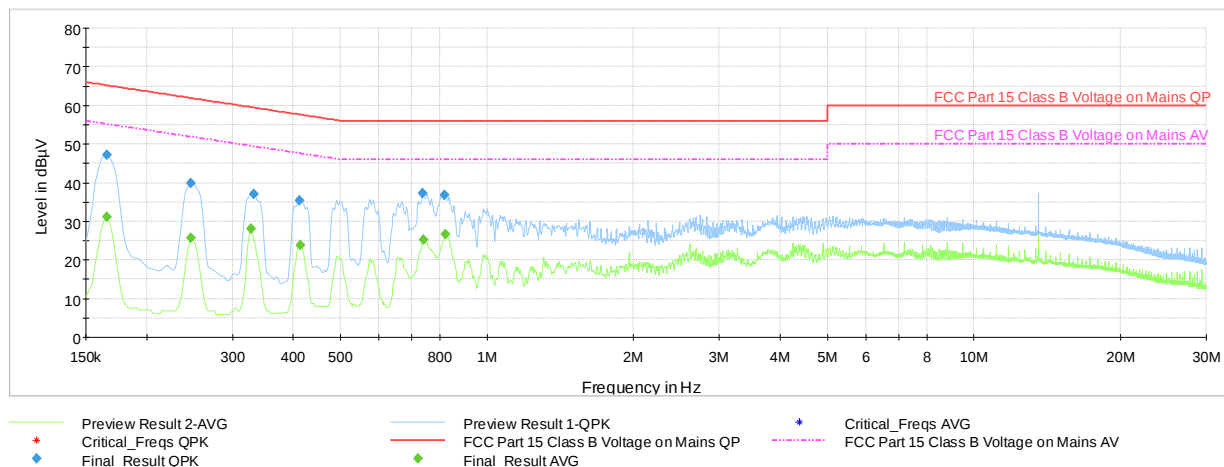
Plot 7-13. AC Line-Conducted Test Plot (N, CE B 848kbps, with WCP + AC/DC Adapter)
