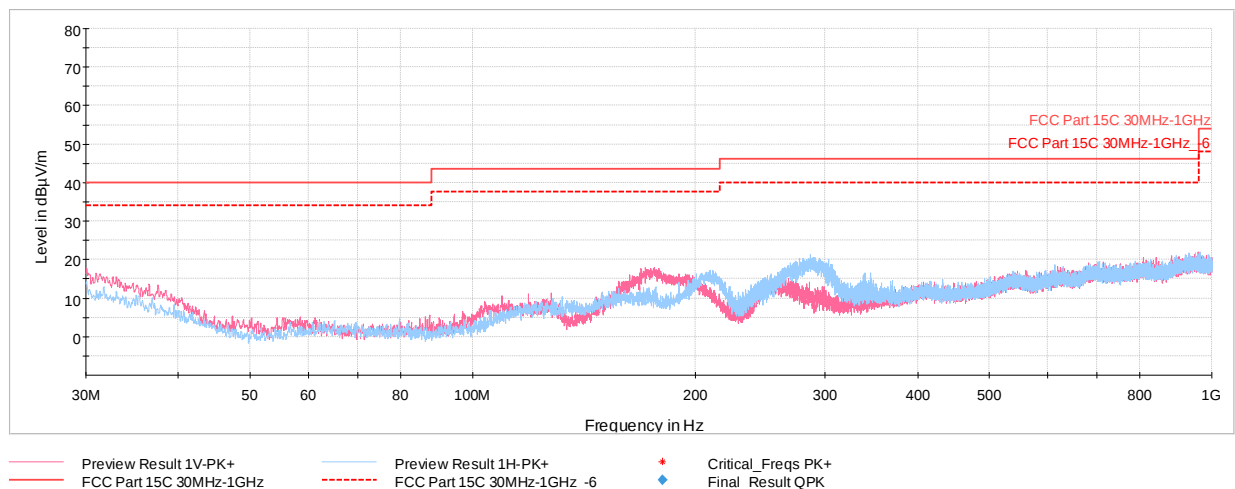
Plot 7-11. Radiated Spurious Emissions 30MHz – 1GHz (Reader 10% Ask 1 out of 4, with WCP + AC/DC Adapter)
