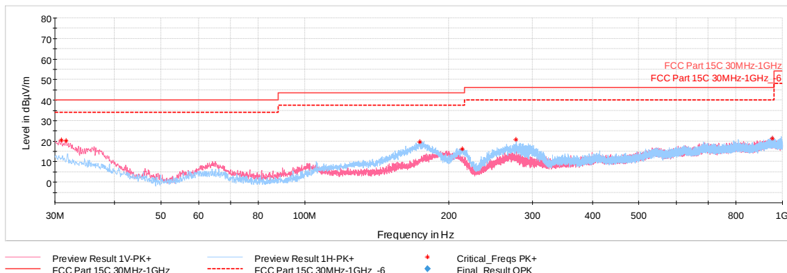
Plot 7-38. Radiated Spurious Emissions 30MHz-1GHz (GFSK ePA – Ch.39, with WCP + AC/DC adapter)
