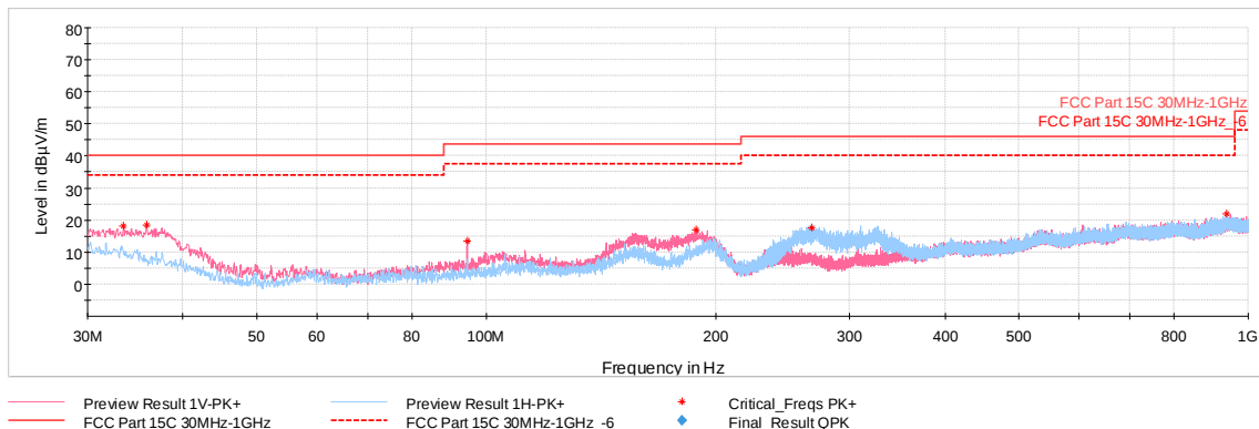
Plot 7-38. Radiated Spurious Emissions 30MHz-1GHz (1Mbps, ePA – Ch.39, with WCP + AC/DC adapter)
