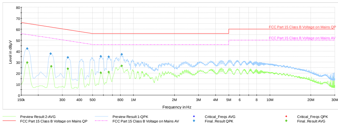
Plot 7-39. AC Line Conducted Emission with Bluetooth LE (L1 - 1Mbps, ePA, Ch.39, with WCP + AC/DC adapter)
