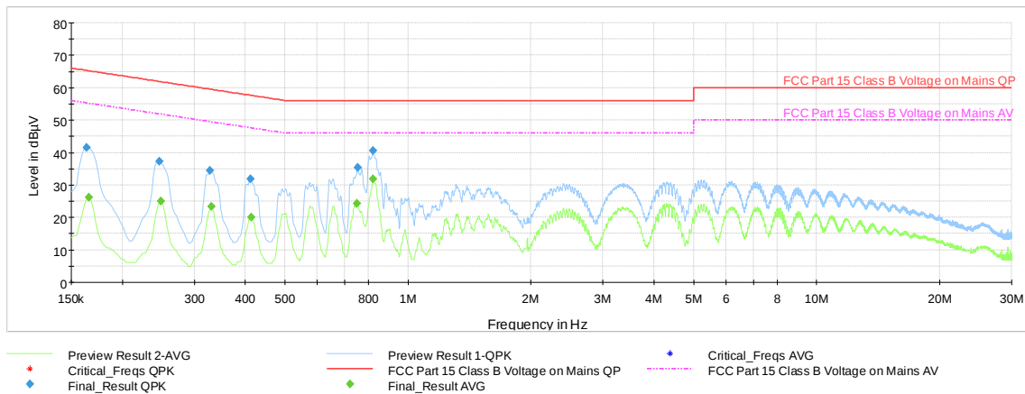
Plot 7-39. AC Line Conducted Emission with Bluetooth HDR (L1 – 4Mbps, ePA, Ch.38, with WCP + AC/DC adapter)
