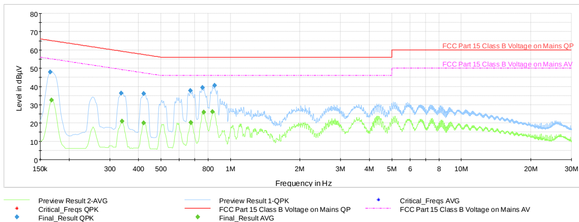
Plot 7-40. AC Line Conducted Emission with Bluetooth HDR (N – 4Mbps, ePA, Ch.38, with WCP + AC/DC adapter)
