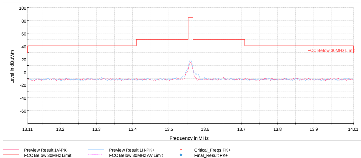
Plot 7-6. In Band Radiated Spurious Emissions (CE A 848kbps, with WCP + AC/DC Adapter)
