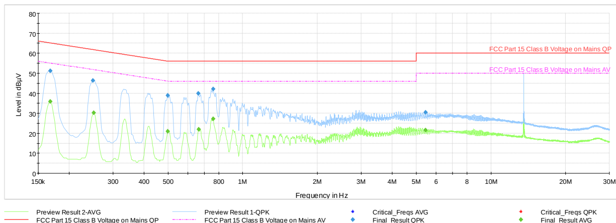
Plot 7-12. AC Line-Conducted Test Plot (L1, with WCP + AC/DC Adapter)
