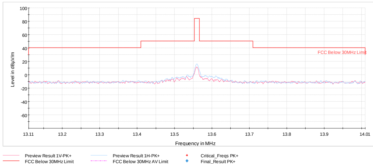
Plot 7-7. In Band Radiated Spurious Emission (Reader 10% Ask 1 out of 256, with WCP + AC/DC Adapter)
