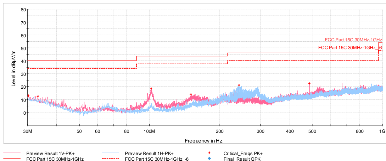
Plot 7-62. Radiated Spurious Emissions 30MHz-1GHz (802.11b – Ch.6, with WCP + laptop)
