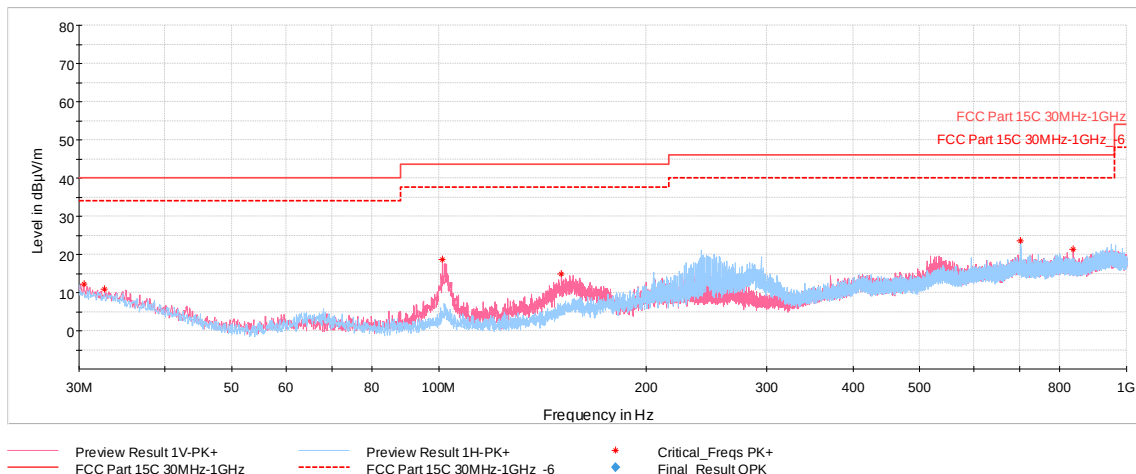
Plot 7-38. Radiated Spurious Emissions 30MHz-1GHz (4Mbps, ePA – Ch.38, with WCP + laptop)
