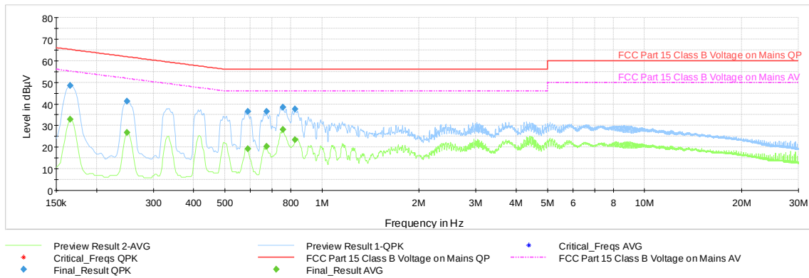
Plot 7-40. AC Line Conducted Plot with Bluetooth HDR (N – 4Mbps, ePA, Ch.38, with WCP + AC/DC Adapter)
