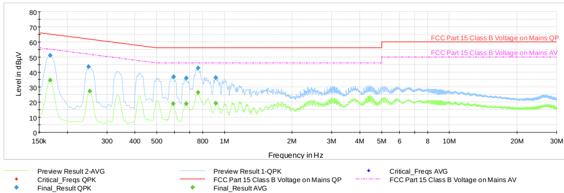
Plot 7-39. AC Line Conducted Plot with Bluetooth HDR (L1 – 4Mbps, ePA, Ch.38, with WCP + AC/DC Adapter)
