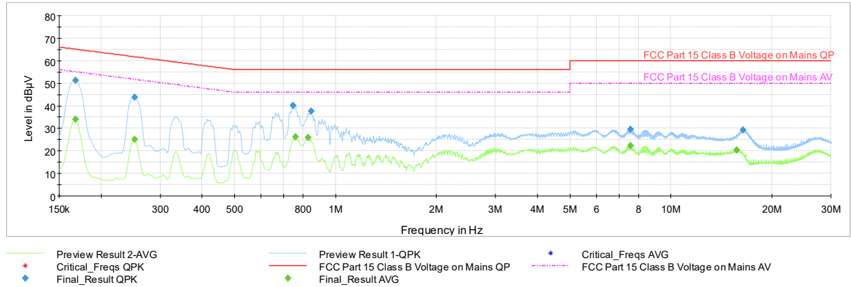
Plot 7-117. AC Line Conducted (Ch. 5, Config 3, Payload 125 L1, with WCP + AC/DC Adapter)
