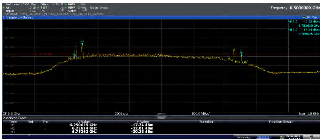
Plot 7-3. 10dBc Bandwidth (Ch. 5, Config 0/Payload 125)
