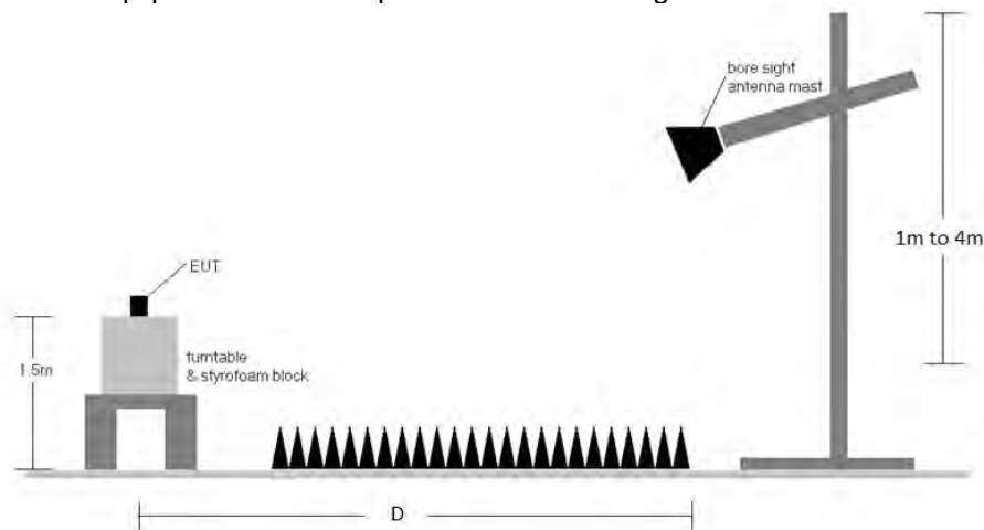
Figure 7-5. Radiated Test Setup - Above 960MHz
