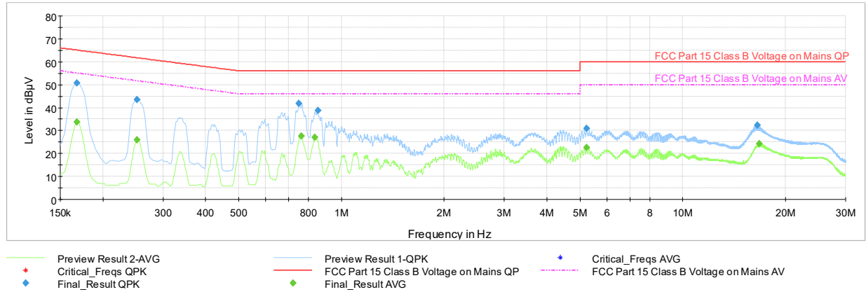
Plot 7-120. AC Line Conducted Plot (Ch. 9, Config 3, Payload 125 N, with WCP + AC/DC Adapter)
