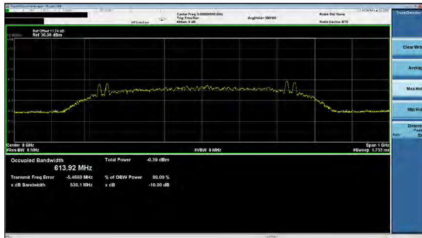
Plot 7-33. ISD Occupied Bandwidth (Ch. 9, Config 0/Payload 125)
