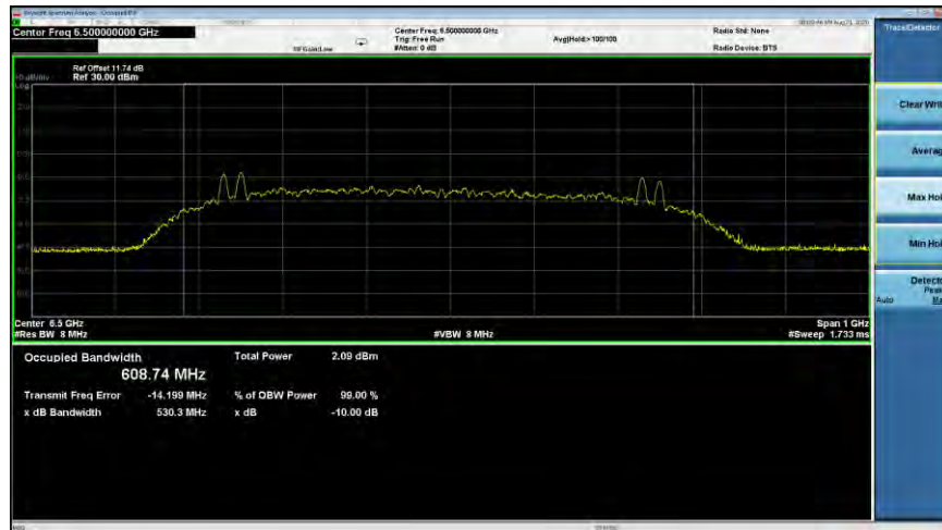
Plot 7-22. ISD Occupied Bandwidth (Ch. 5, Config 0/Payload 65)
