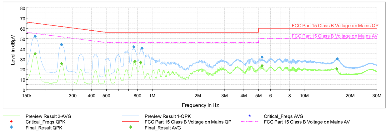
Plot 7-119. AC Line Conducted (Ch. 9, Config 3, Payload 125 L1, with WCP + AC/DC Adapter)
