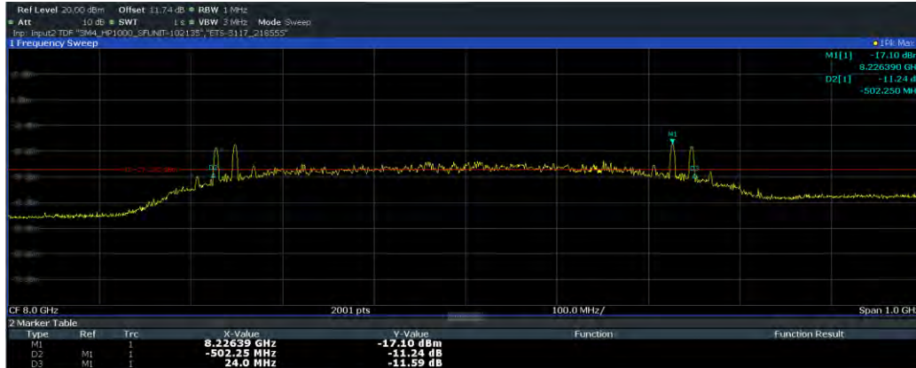
Plot 7-11. 10dBc Bandwidth (Ch. 9, Config 0/Payload 25)
