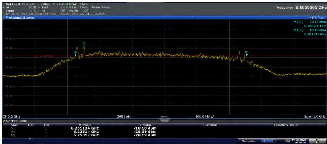
Plot 7-10. 10dBc Bandwidth (Ch. 5, Config 5/Payload 0)
