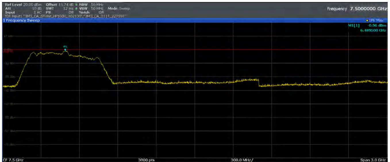
Plot 7-44. Peak Radiated Power (Ch. 5, Config 1/Payload 45)
