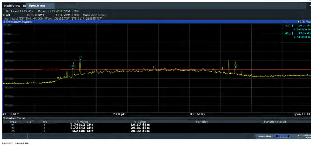
Plot 7-17. 10dBc Bandwidth (Ch. 9, Config 2/Payload 125)
