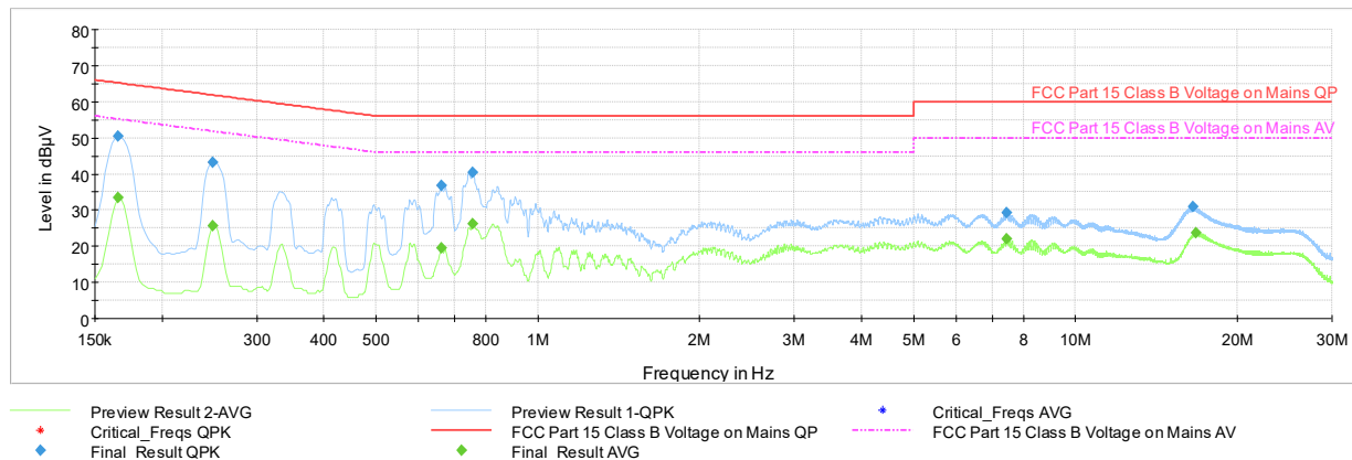
Plot 7-118. AC Line Conducted (Ch. 5, Config 3, Payload 125 N, with WCP + AC/DC Adapter)
