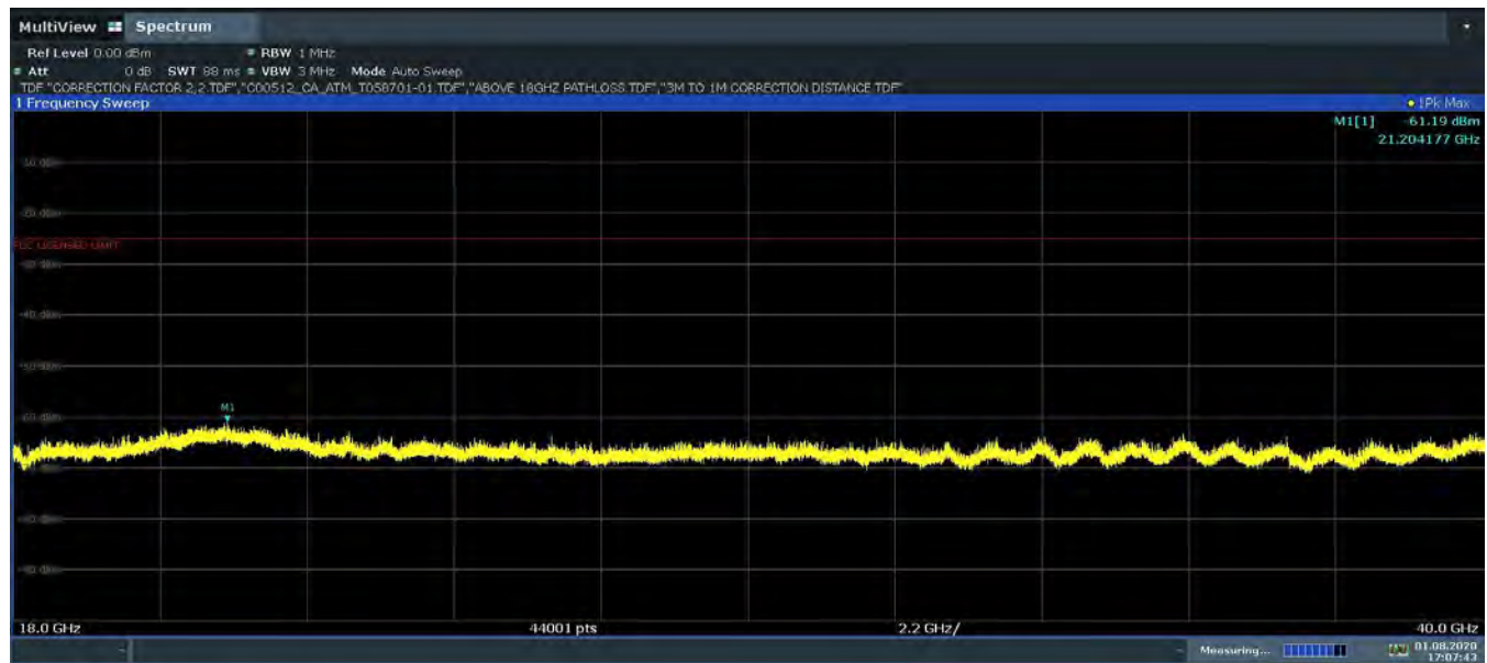
Plot 7-112. Radiated Spurious Emission- Simultaneous Transmission 18GHz-40GHz Pol. H
