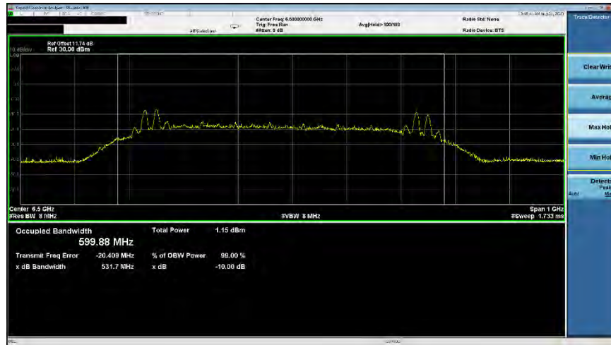
Plot 7-30. ISED Occupied Bandwidth (Ch. 5, Config 5/Payload 0)
