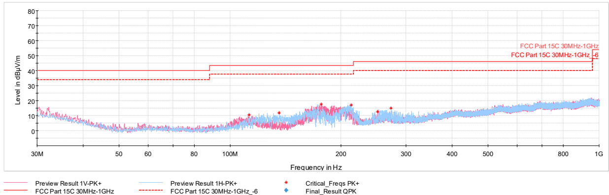
Plot 7-116. Radiated Spurious Emission – Simultaneous Transmission below 960 MHz with WCP + AC/DC Adapter
