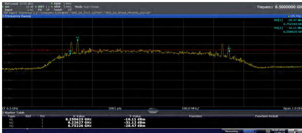
Plot 7-5. 10dBc Bandwidth (Ch. 5, Config 1/Payload 85)
