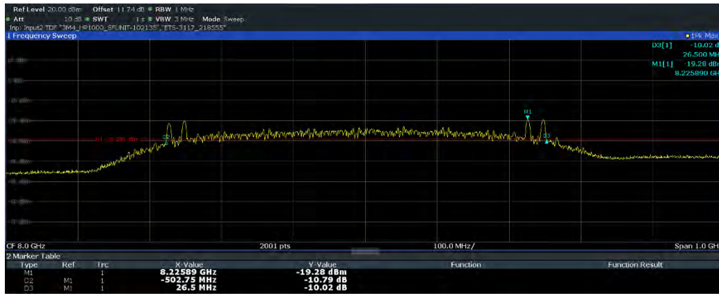
Plot 7-20. 10dBc Bandwidth (Ch. 9, Config 5/Payload 0)
