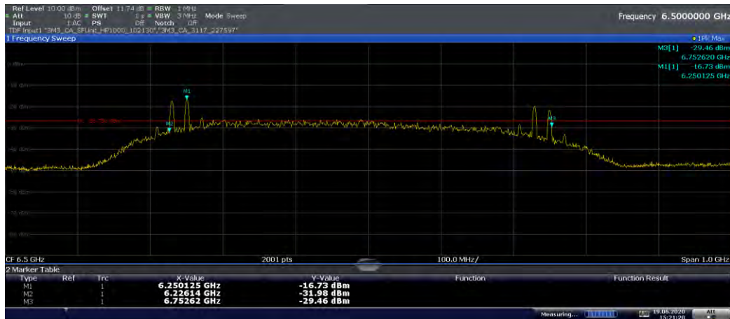
Plot 7-2. 10dBc Bandwidth (Ch. 5, Config 0/Payload 65)
