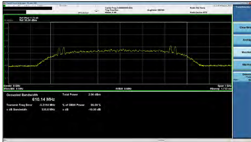
Plot 7-31. ISD Occupied Bandwidth (Ch. 9, Config 0/Payload 25)
