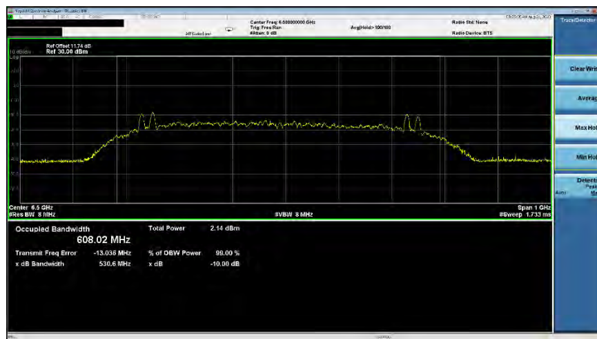
Plot 7-21. ISD Occupied Bandwidth (Ch. 5, Config 0/Payload 25)
