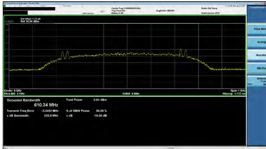
Plot 7-32. ISD Occupied Bandwidth (Ch. 9, Config 0/Payload 65)
