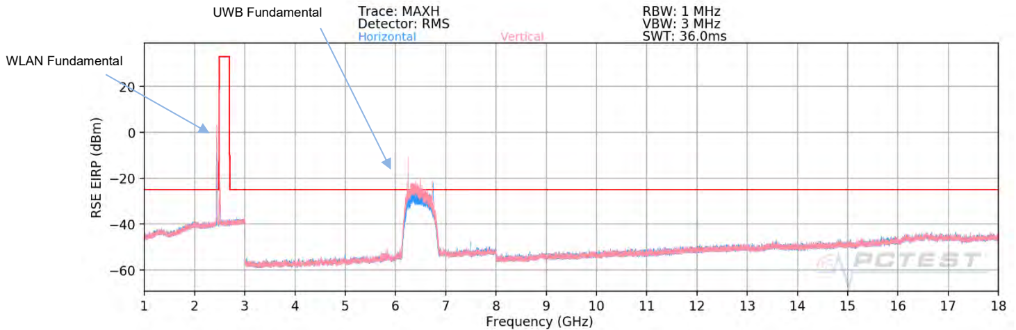
Plot 7-111. Radiated Spurious Simultaneous TX 1-18GHz (Ch. 5, Config 3, Payload 125)
