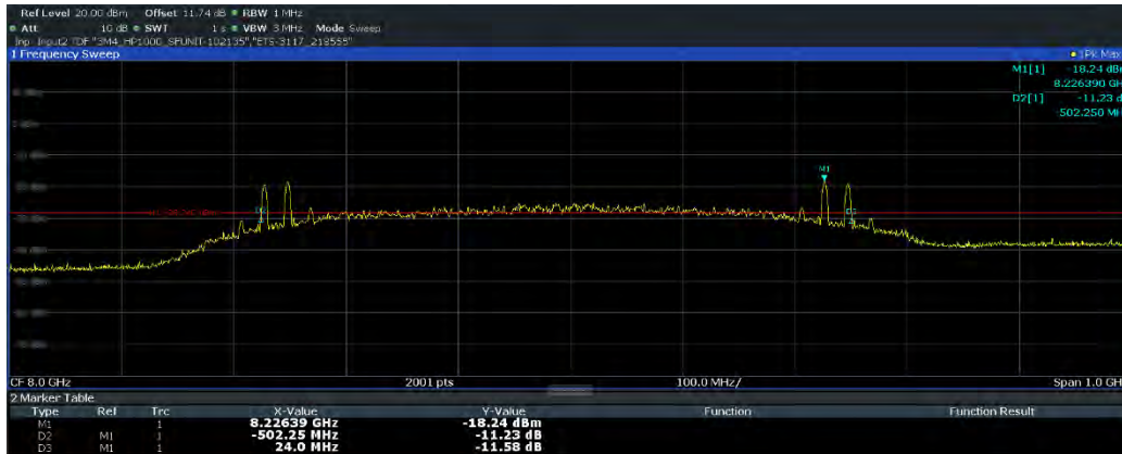
Plot 7-12. 10dBc Bandwidth (Ch. 9, Config 0/Payload 65)
