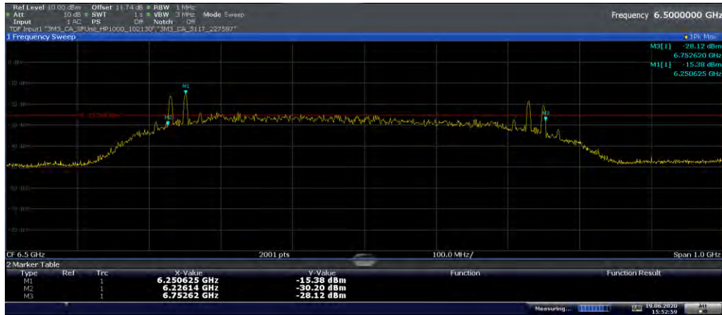
Plot 7-1. 10dBc Bandwidth (Ch. 5, Config 0/Payload 25)
