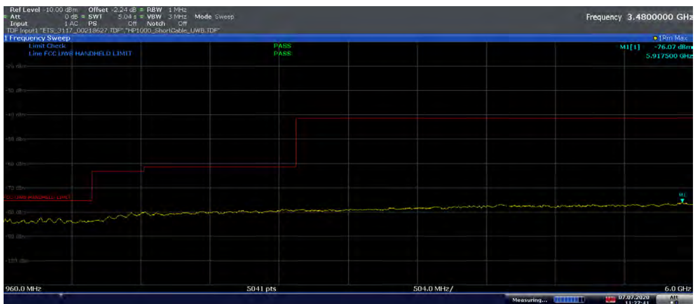
Plot 7-98. FCC Radiated Spurious Emission 960-6000MHz (Ch.9, Config 3, Payload 125 Ant. Pol. V)
