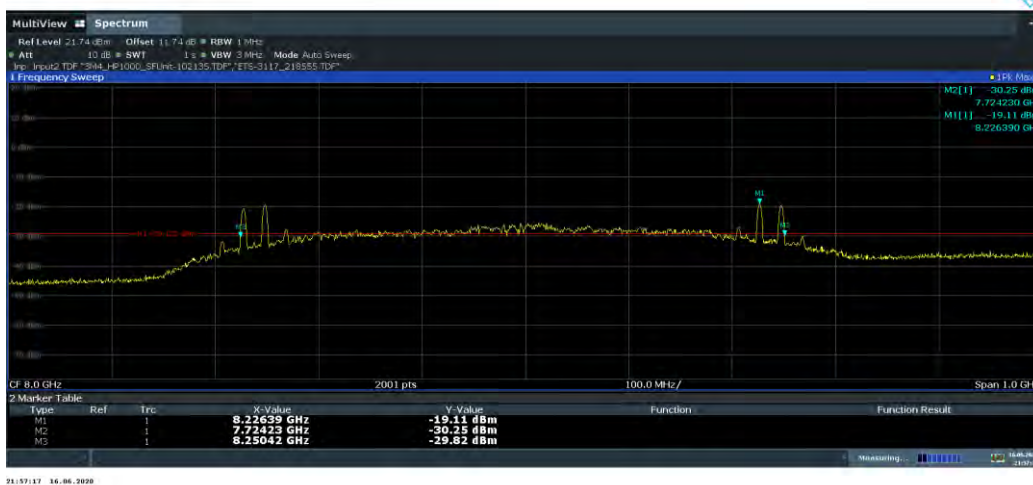
Plot 7-16. 10dBc Bandwidth (Ch. 9, Config 1/Payload 125)
