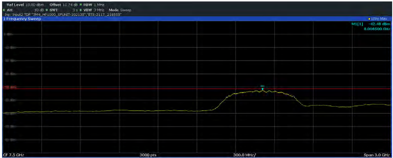
Plot 7-80. Average Radiated Power (Ch. 9, Config 5/Payload 0)
