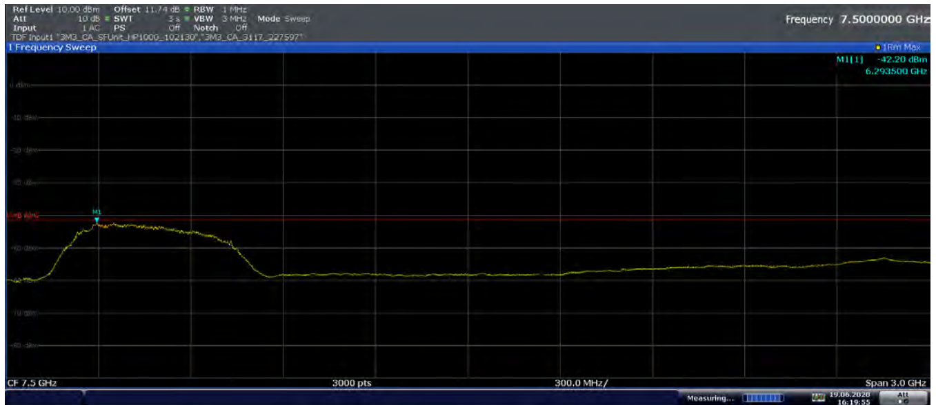
Plot 7-69. Average Radiated Power (Ch. 5, Config 4/Payload 0)
