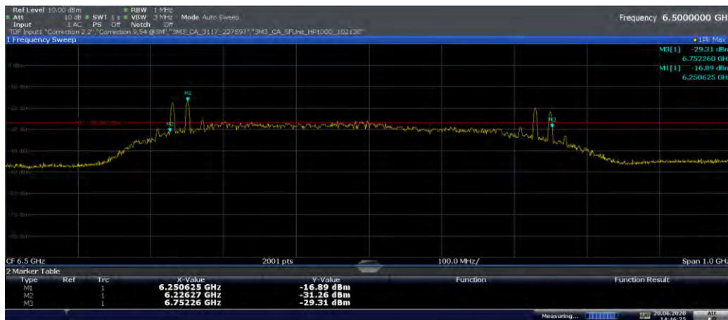
Plot 7-6. 10dBc Bandwidth (Ch. 5, Config 1/Payload 125)
