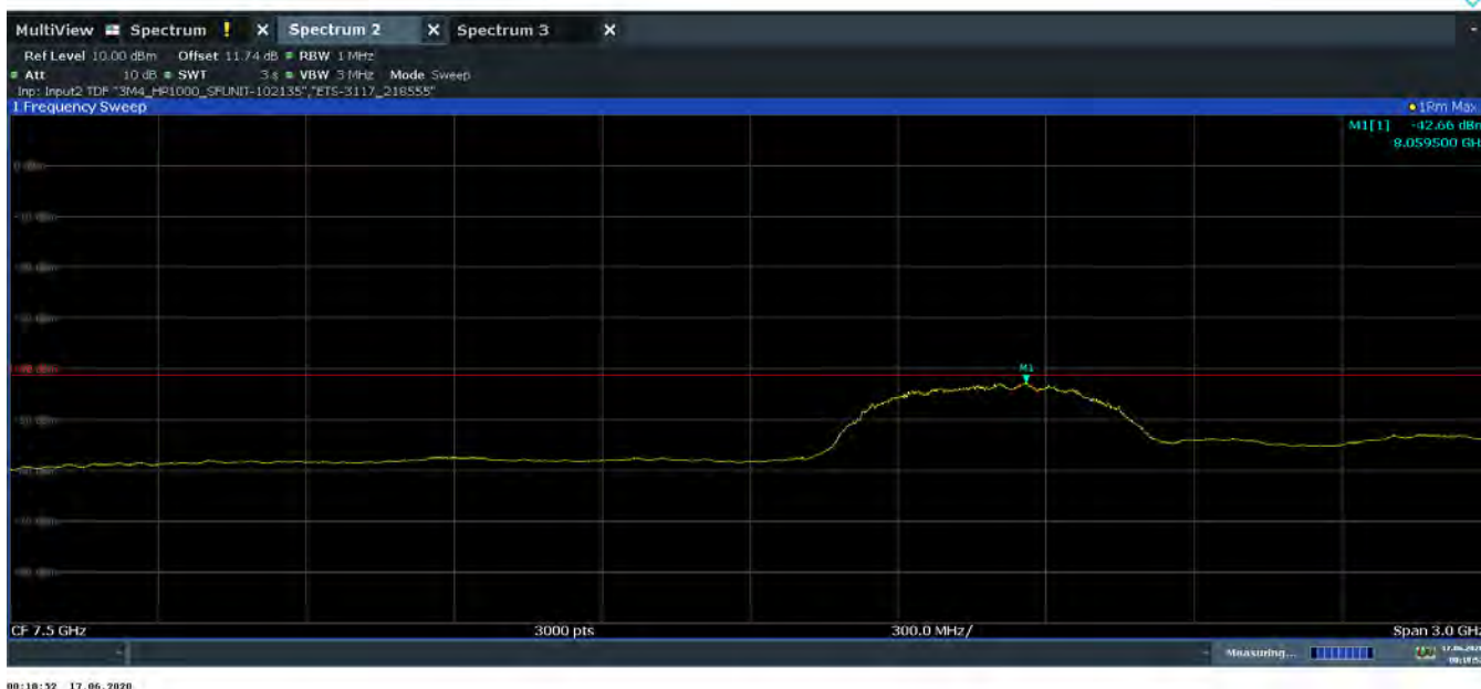
Plot 7-73. Average Radiated Power (Ch. 9, Config 0/Payload 125)
