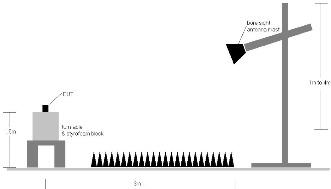
Figure 7-1. Test Setup
