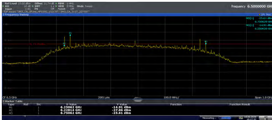
Plot 7-8. 10dBc Bandwidth (Ch. 5, Config 3/Payload 125)
