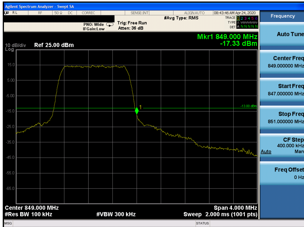
Plot 7-145. Upper Band Edge Plot (Band 26 - 1.4MHz QPSK - Full RB Configuration)
