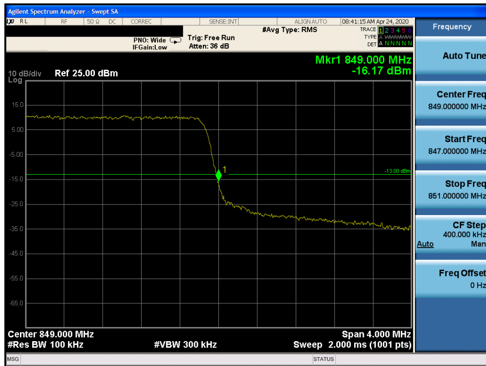
Plot 7-147. Upper Band Edge Plot (Band 26 - 3.0MHz QPSK - Full RB Configuration)
