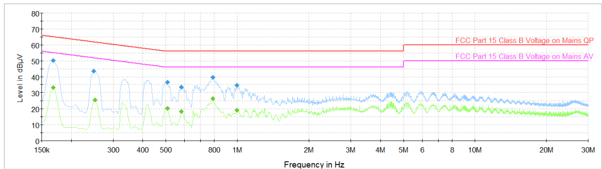
Plot 7-39. AC Line-Conducted Plot – GFSK ePA Ch.39 (L1, with WCP + AC/DC Adapter)
