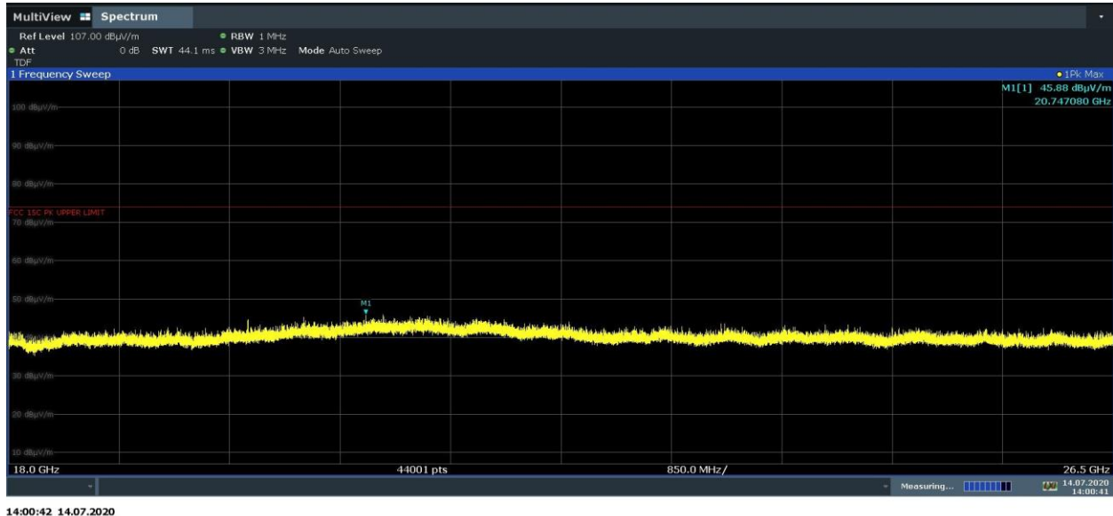
Plot 7-32. Radiated Spurious Emissions 18-26.5GHz (GFSK ePA – Ch.39, Pol. H)
