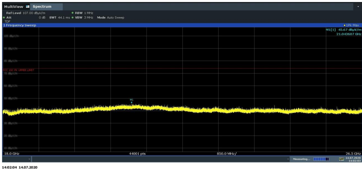
Plot 7-33. Radiated Spurious Emissions 18-26.5GHz (GFSK ePA – Ch.39, Pol. V)
