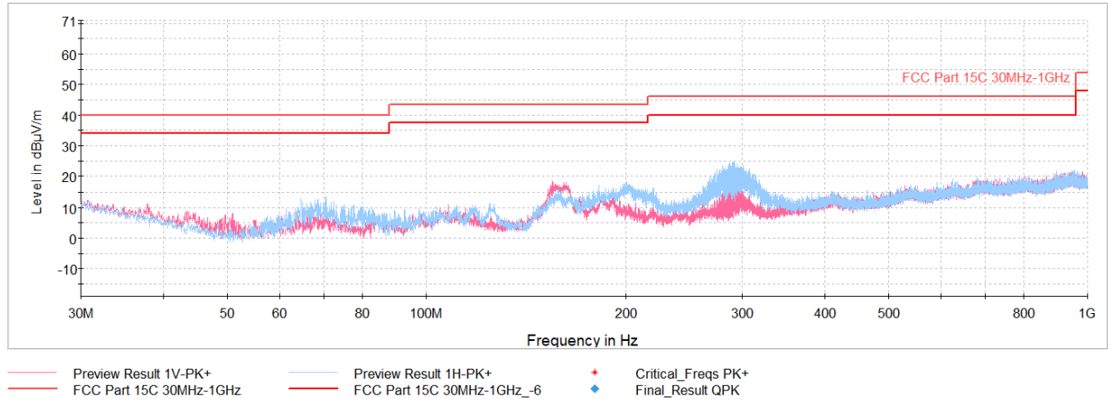
Plot 7-38. Radiated Spurious Emissions 30MHz-1GHz (GFSK ePA – Ch.39, with WCP + Laptop)
