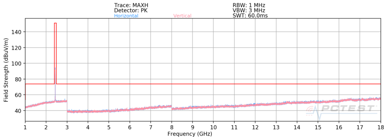
Plot 7-44. Radiated Spurious Emissions 1-18GHz (802.11b – Ch. 6)
