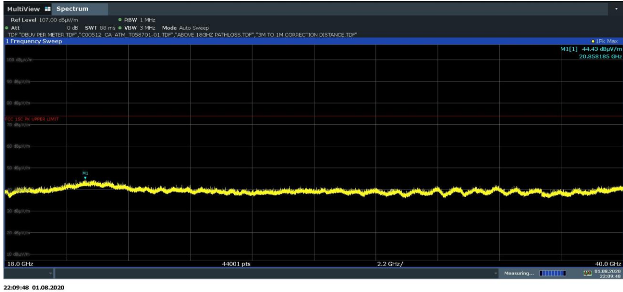
Plot 7-50. Radiated Spurious Emissions 18-40GHz (Simultaneous Transmission, Ant. Pol. V)
