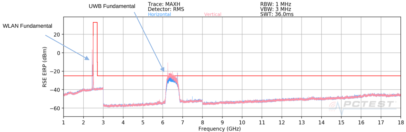
Plot 7-48. Radiated Spurious Emissions 1-18GHz (Simultaneous Transmission)
