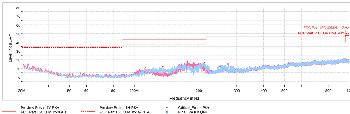
Plot 7-63. Radiated Spurious Emissions 30MHz-1GHz (Simultaneous Transmission, with WCP + AC/DC adapter)
