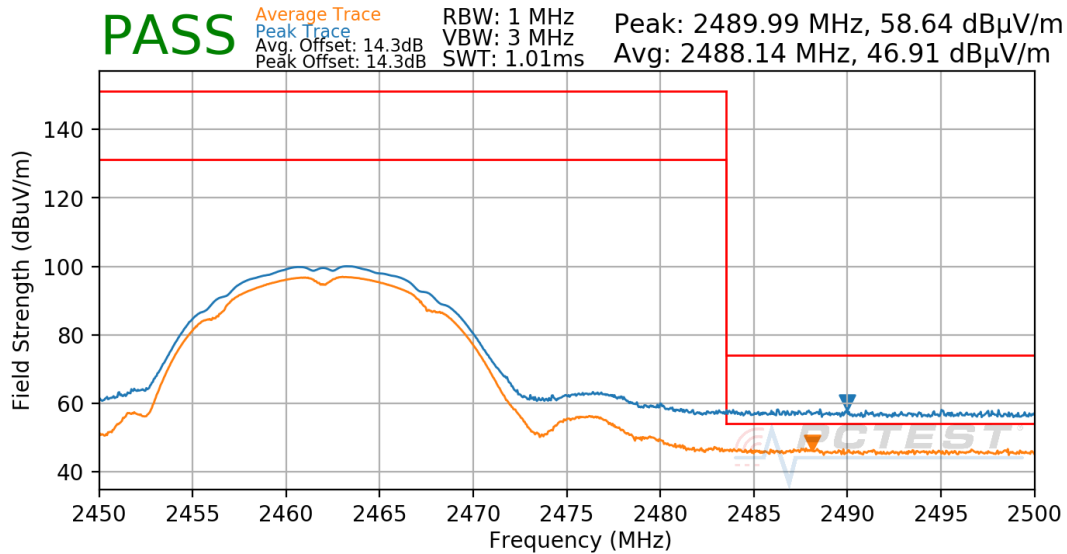
Plot 7-52. Radiated Restricted Upper Band Edge Measurement
