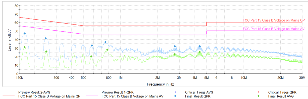
Plot 7-65. AC Line Conducted Plot with 802.11b Ch.6 (N, with WCP + AC/DC Adapter)
