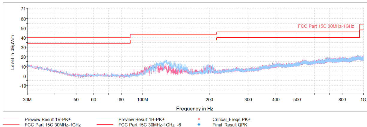
Plot 7-62. Radiated Spurious Emissions 30MHz-1GHz (802.11b – Ch.6, with WCP + AC/DC Adapter)
