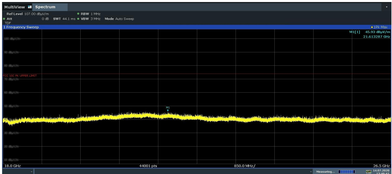
Plot 7-47. Radiated Spurious Emissions 18-26.5GHz (802.11b – Ch. 6, Ant. Pol. V)
