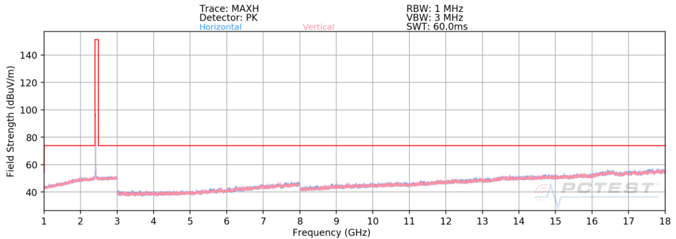
Plot 7-43. Radiated Spurious Emissions 1-18GHz (802.11b – Ch. 1)
