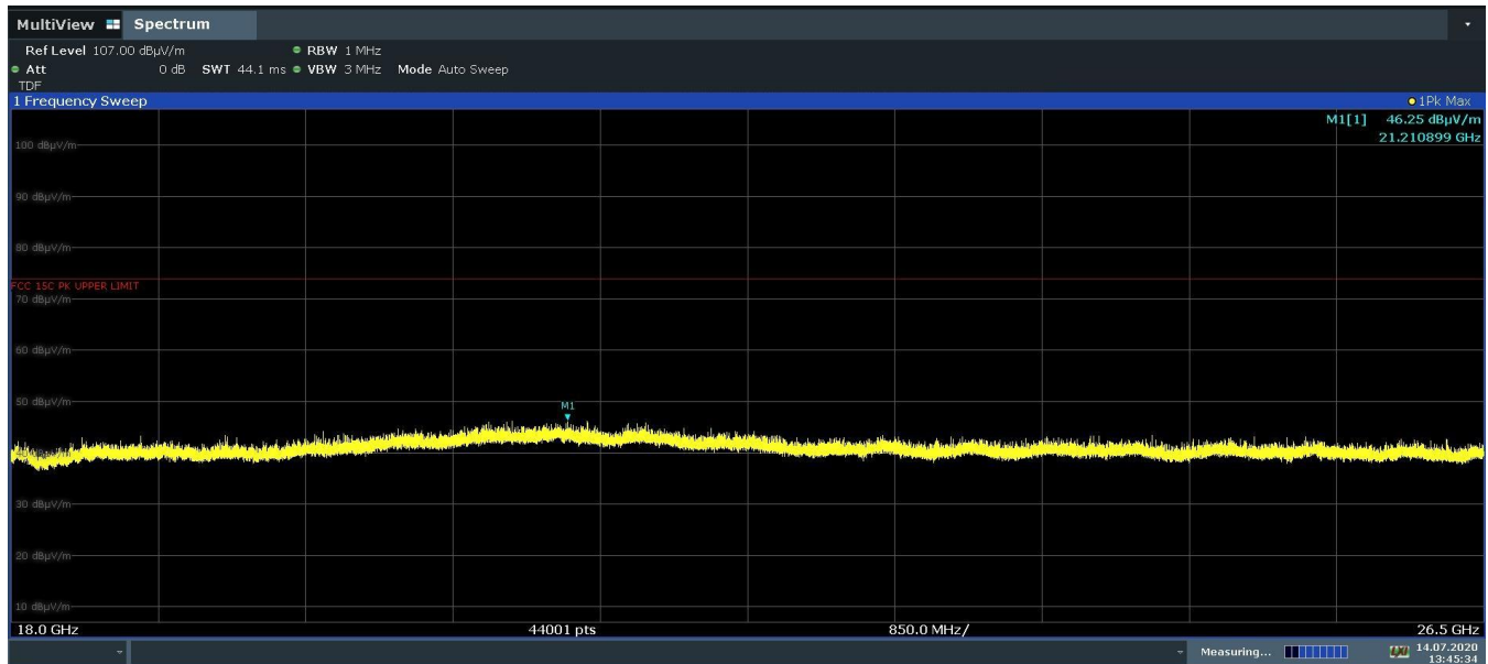
Plot 7-46. Radiated Spurious Emissions 18-26.5GHz (802.11b – Ch. 6, Ant. Pol. H)
