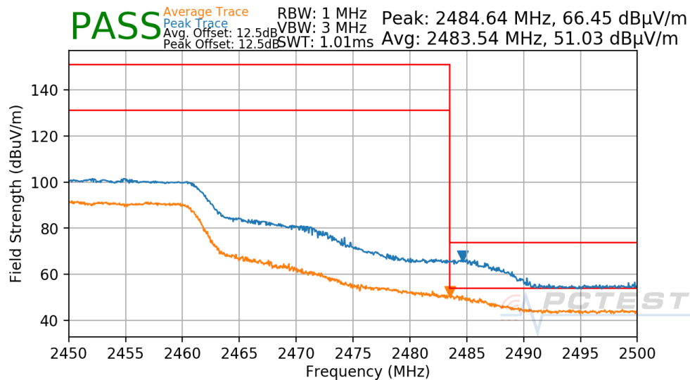
Plot 7-57. Radiated Restricted Upper Band Edge Measurement
