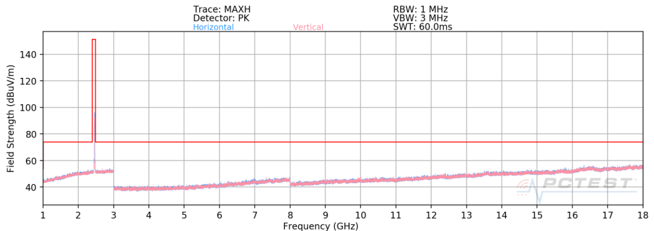
Plot 7-45. Radiated Spurious Emissions 1-18GHz (802.11b – Ch. 11)
