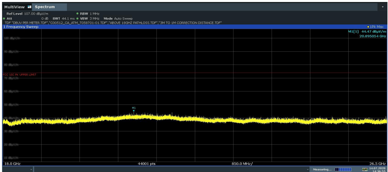
Plot 7-33. Radiated Spurious Emissions 18-26.5GHz (4Mbps, HDR4, ePA – Ch.38, Ant. Pol. V)
