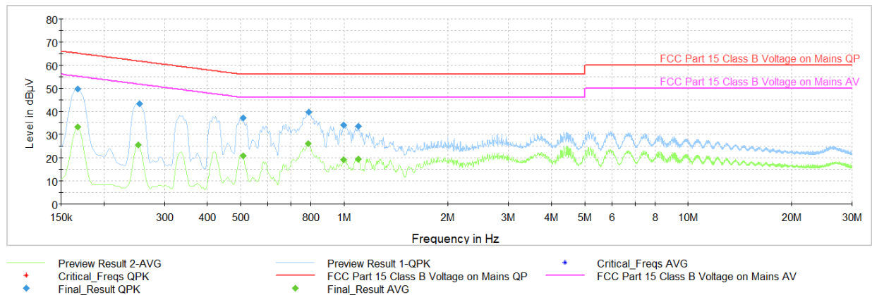
Plot 7-39. AC Line Conducted Plot with Bluetooth HDR (L1 - 4Mbps, ePA, Ch.38 with WCP + AC/DC Adapter)
