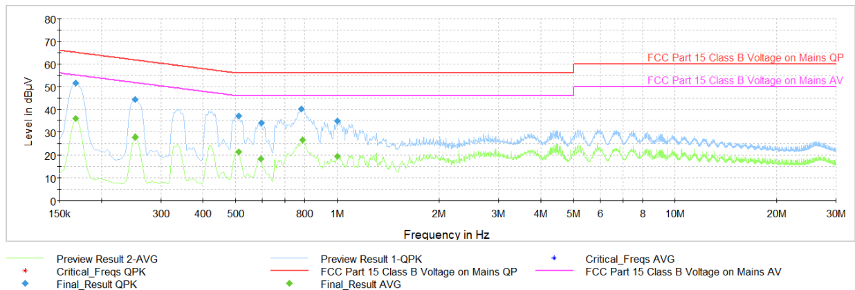
Plot 7-39. AC Line Conducted Plot with Bluetooth LE (1Mbps, ePA – Ch.19, L1, with WCP + AC/DC Adapter)
