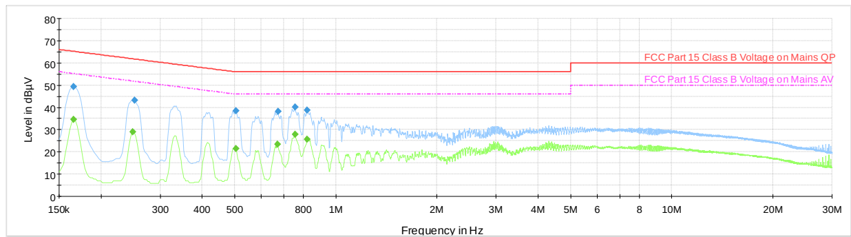
Plot 7-48. AC Line Conducted Plot with 802.11n UNII Band 1 – Ch.36 (N) with AC/DC Adapter
