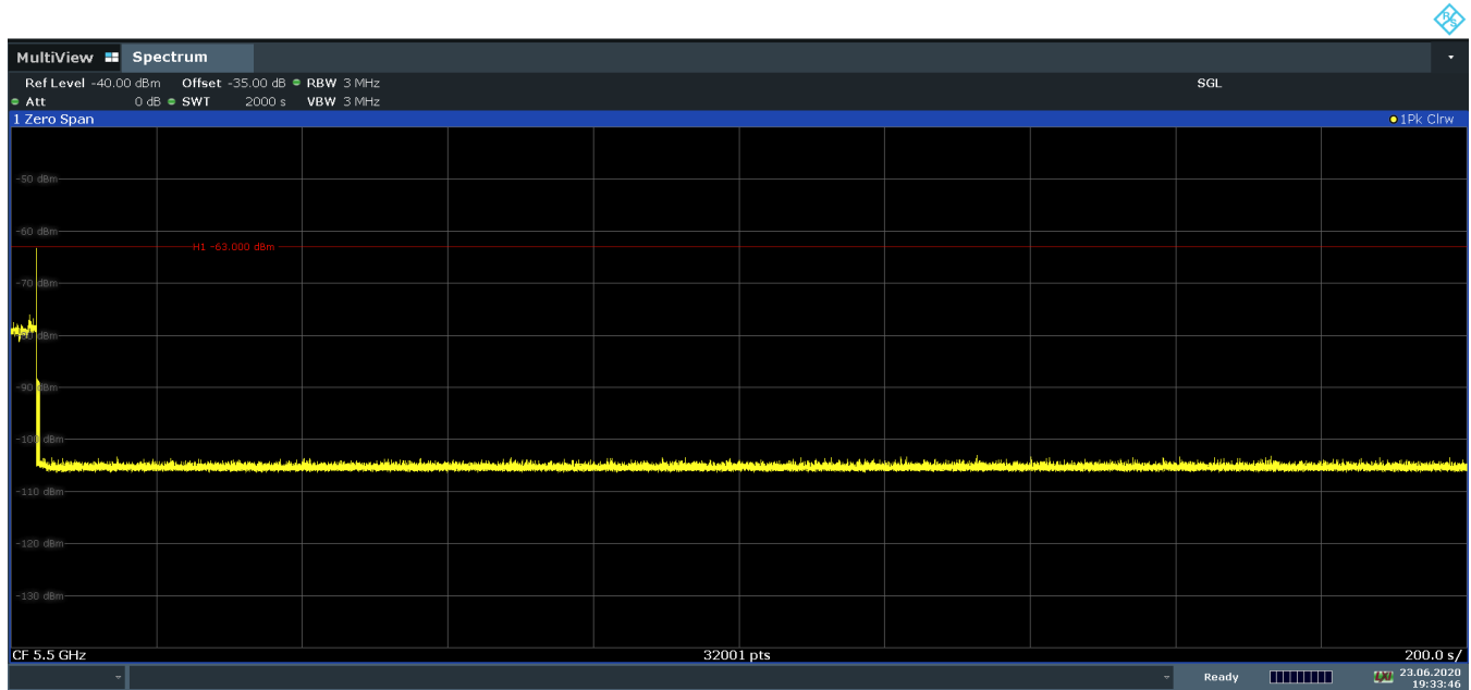
Figure 9-4. 5500MHz - Non-Occupancy Period (30 Minutes) - (20MHz)
