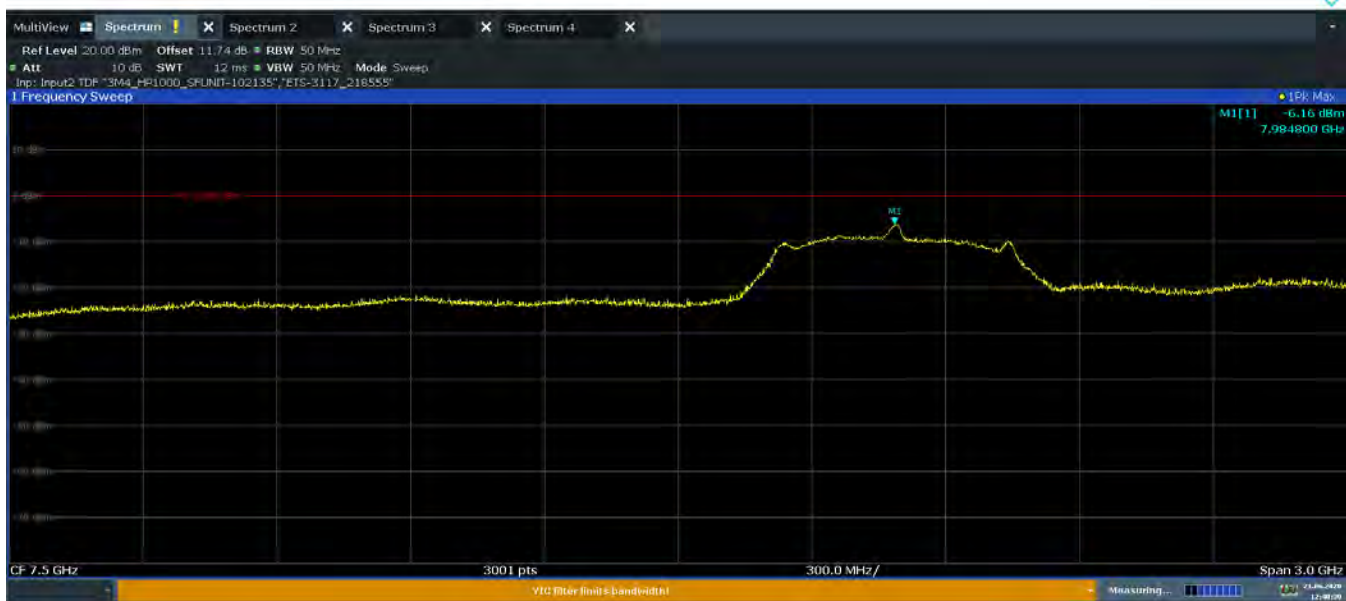
Plot 7-58. Peak Radiated Power (Ch. 9, Config 3/Payload 125)
