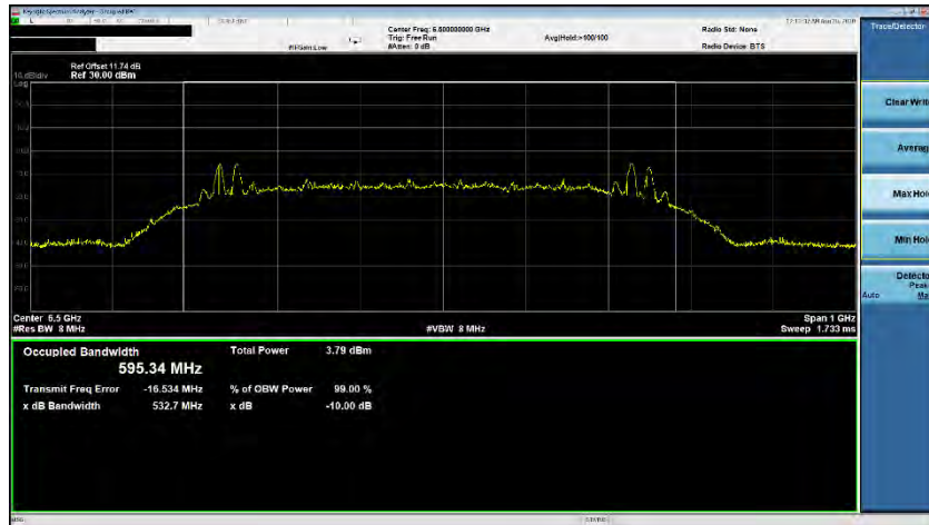
Plot 7-30. ISCED Occupied Bandwidth (Ch. 5, Config 5/Payload 0)
