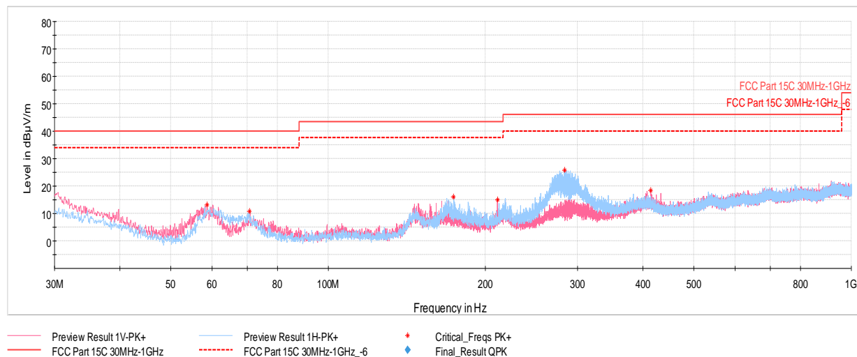
Plot 7-49. Radiated Spurious Emissions below 1GHz (802.11n – UNII 2C Ch. 100) with WCP + laptop
