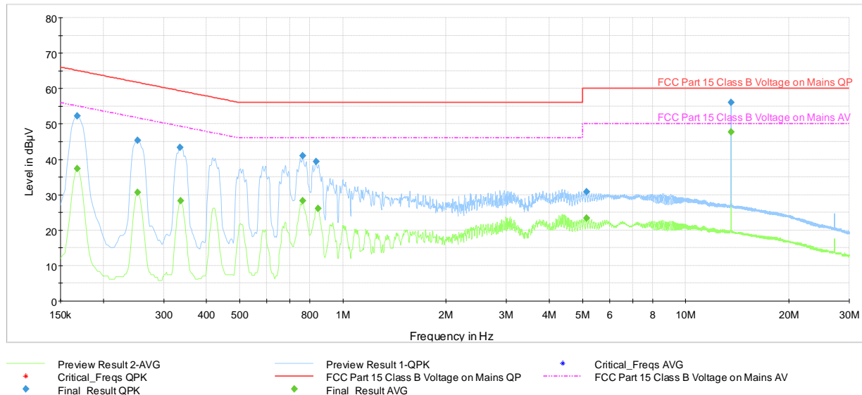
Plot 7-13. AC Line-Conducted Test Plot (N, with WCP + AC/DC Adapter)
