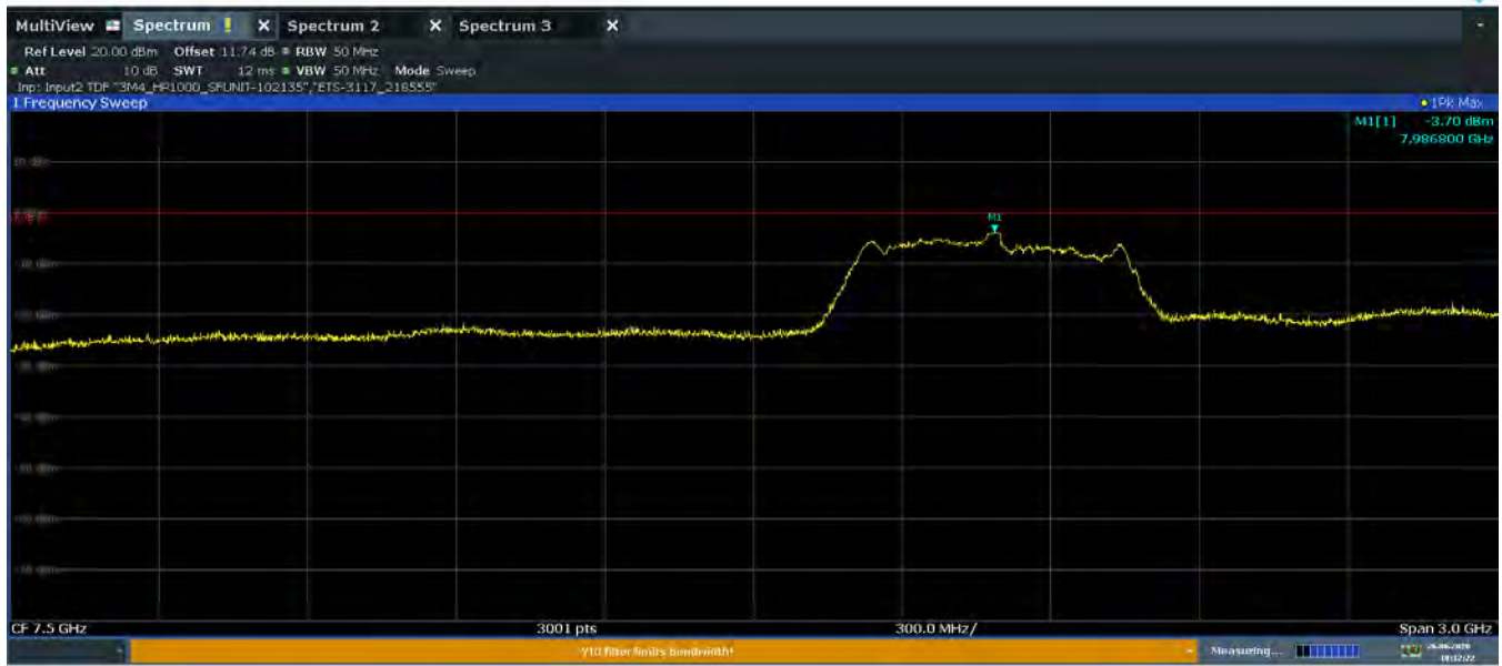
Plot 7-53. Peak Radiated Power (Ch. 9, Config 0/Payload 125)
