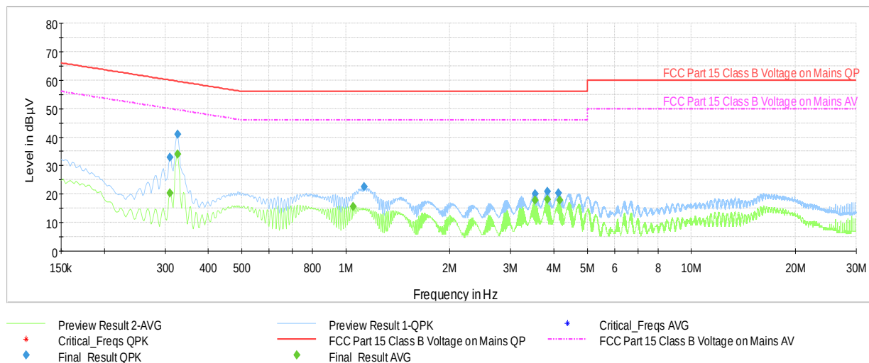
Plot 7-51. AC Line Conducted Plot with 802.11n UNII Band 3 – Ch.165 (L1) with Laptop
