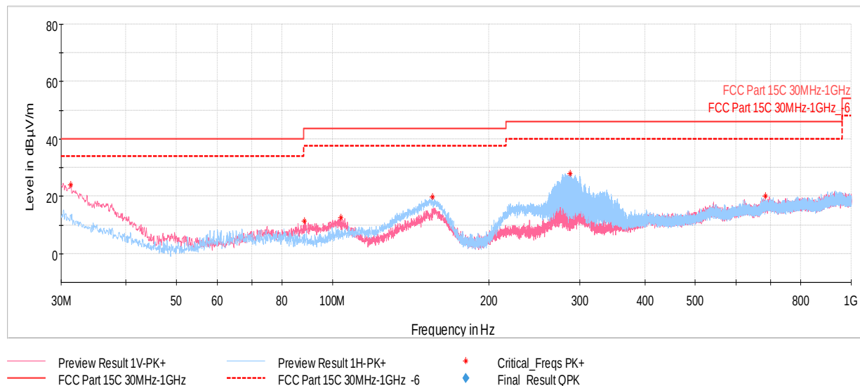
Plot 7-49. Radiated Spurious Emissions below 1GHz (802.11n – UNII 3 Ch. 165) with AC/DC adapter
