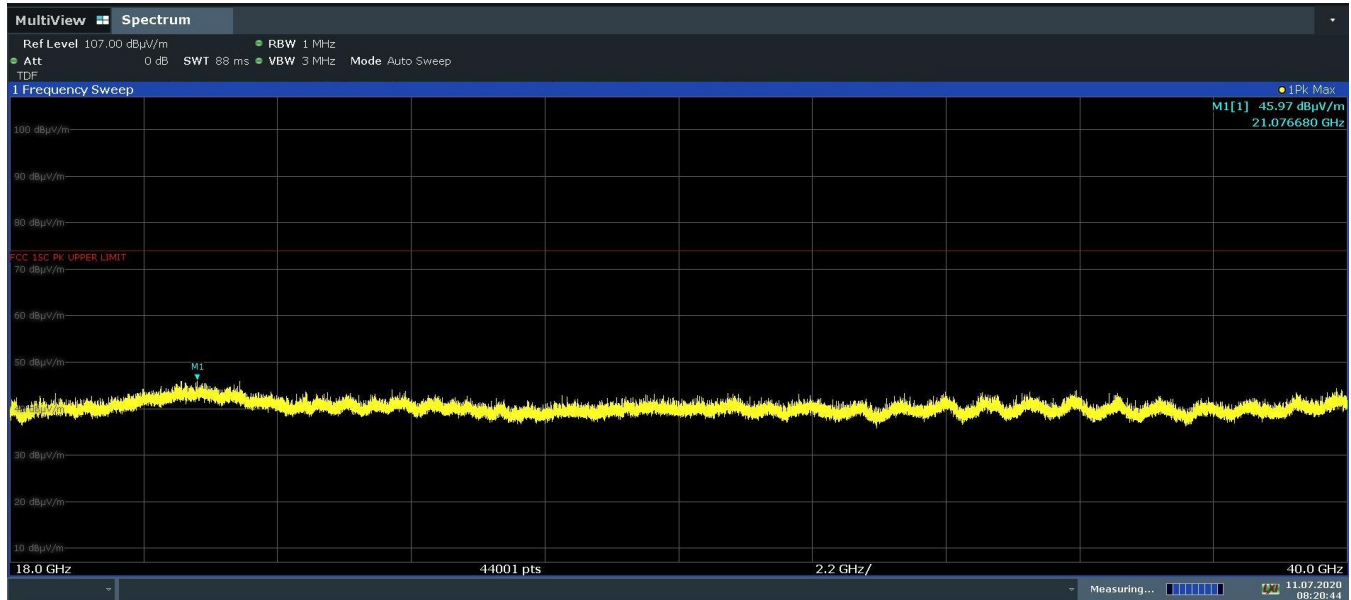
Plot 7-37. Radiated Spurious Emissions 18GHz - 40GHz – H Polarity (802.11n Ch 165)
