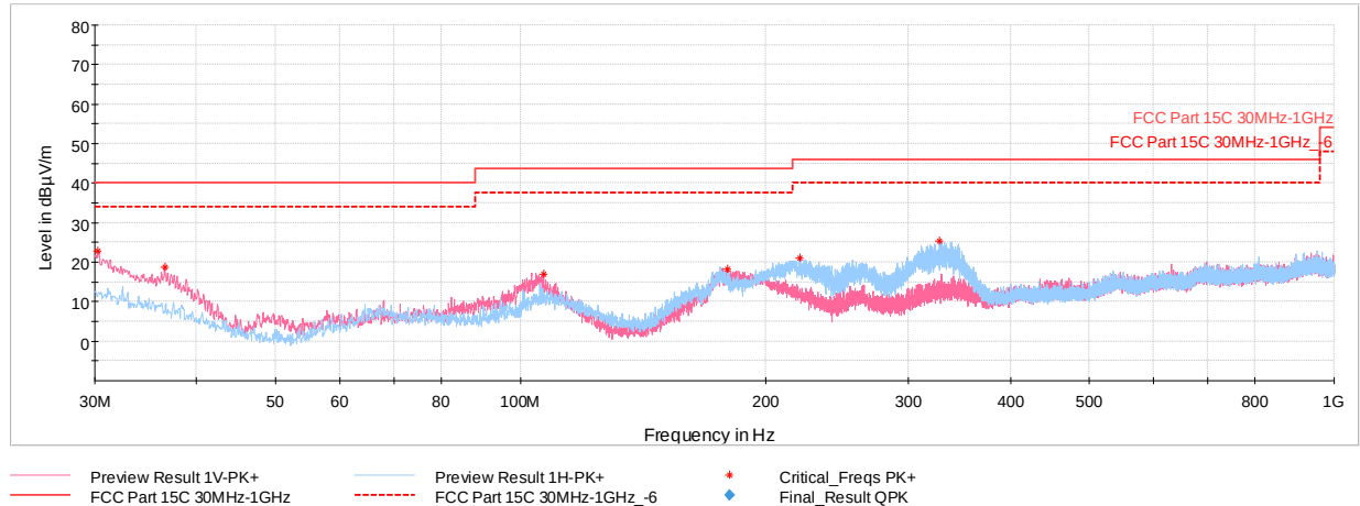
Plot 7-50. Radiated Spurious Emission – Simultaneous Transmission below 1GHz with AC/DC Adapter
