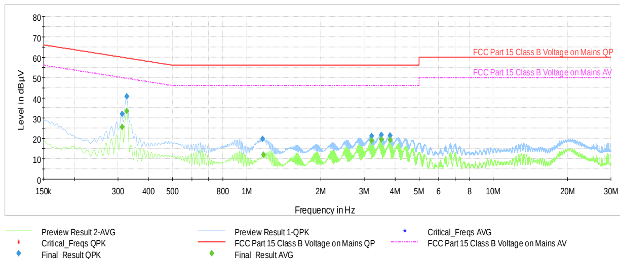
Plot 7-52. AC Line Conducted Plot with 802.11n UNII Band 3 – Ch.165 (N) with Laptop
