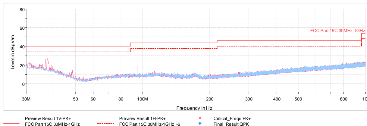
Plot 7-42. Radiated Spurious Plot Below 1GHz (with WCP + AC/DC Adapter)
