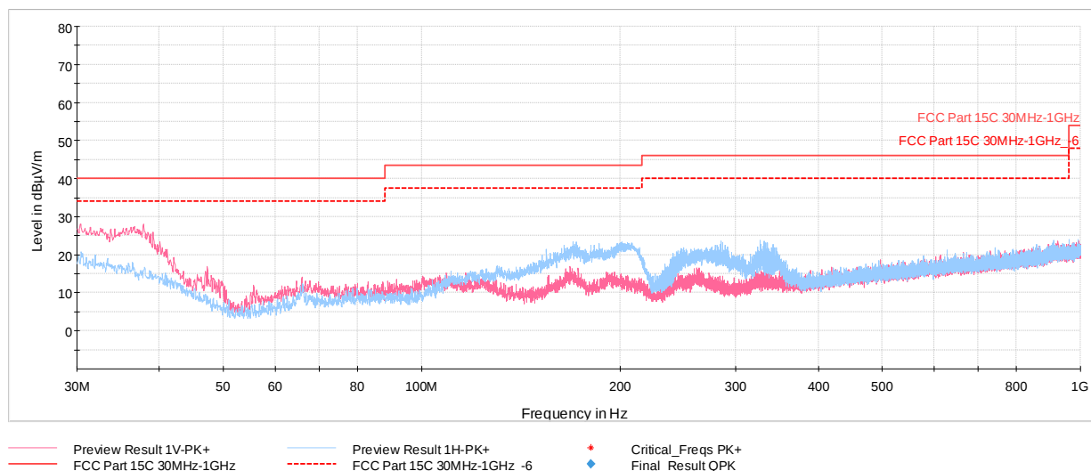
Plot 7-38. Radiated Spurious Plot below 1GHz (4Mbps, ePA – Ch.38 with WCP + AC/DC Adapter attached)
