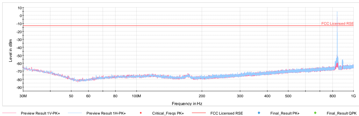
Plot 7-22. Radiated Spurious Plot - Below 1GHz (LTE Band 26 High channel, with WCP + AC/DC Adapter)
