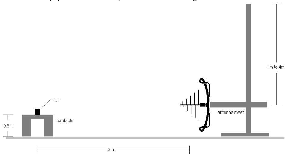
Figure 7-5. Test Instrument & Measurement Setup for < 1 GHz
