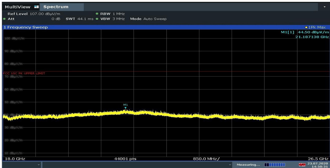
Plot 7-33. Radiated Spurious Emissions 18-26.5GHz (GFSK iPA – Ch.39, Pol. V)
