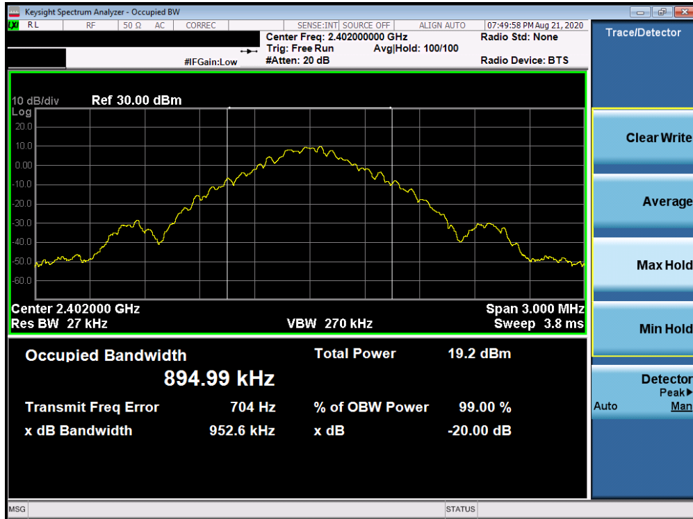
Plot 7-1. 20dB BW / 99% OBW Plot (Bluetooth, GFSK, iPA – Ch. 0)
