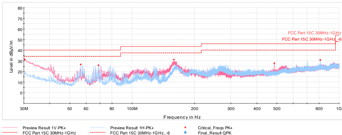
Plot 7-38. Radiated Spurious Emissions 30MHz-1GHz (GFSK iPA – Ch.39, with Laptop)
