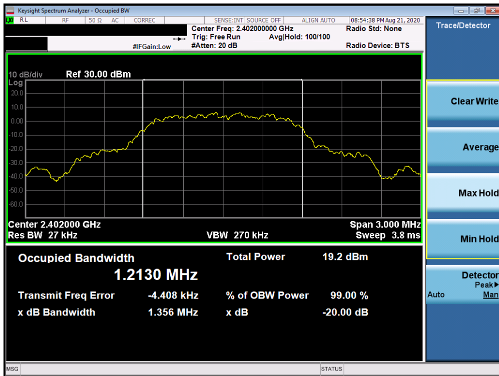
Plot 7-4. 20dB BW / 99% OBW Plot (Bluetooth, 8DPSK, iPA – Ch. 0)
