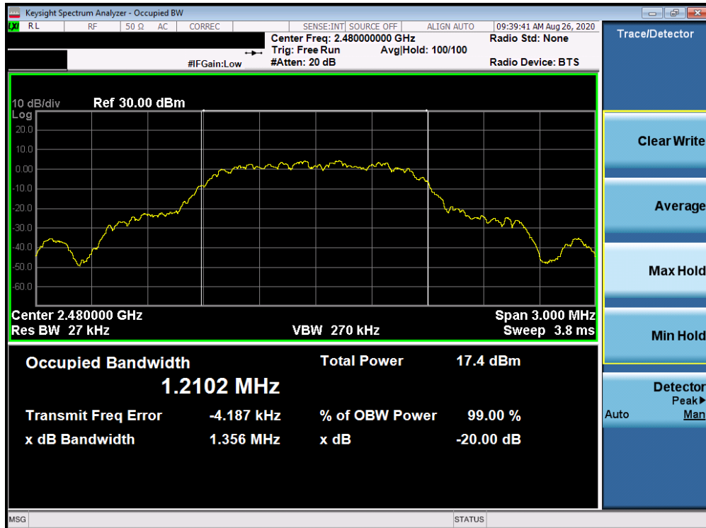
Plot 7-6. 20dB BW / 99% OBW Plot (Bluetooth, 8DPSK, iPA – Ch. 78)
