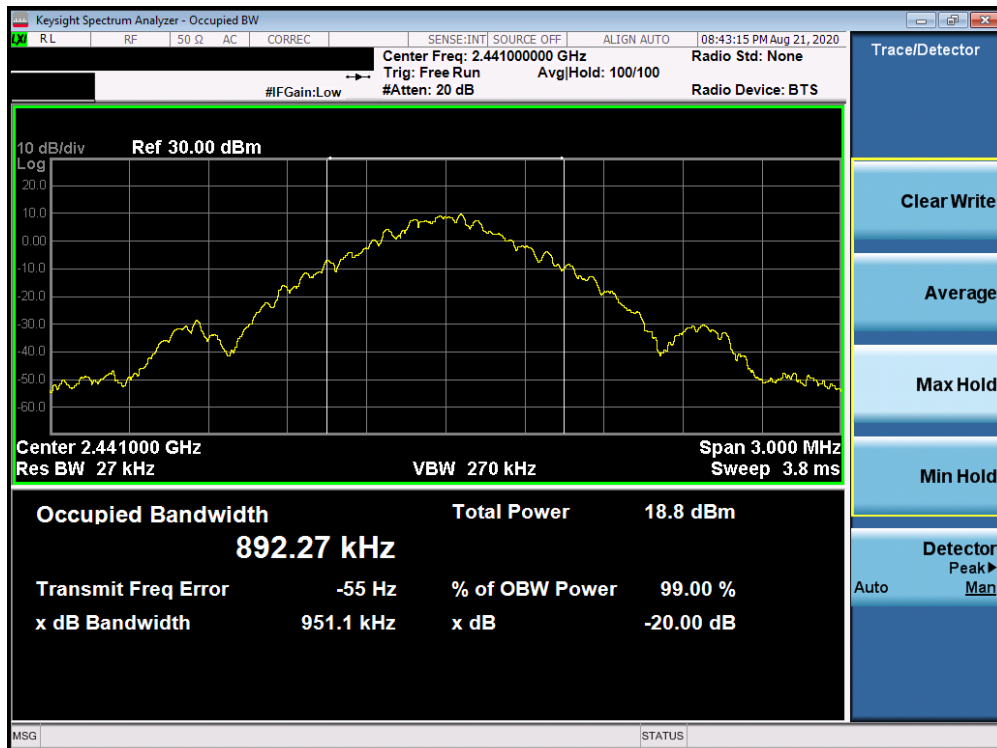
Plot 7-2. 20dB BW / 99% OBW Plot (Bluetooth, GFSK, iPA – Ch. 39)
