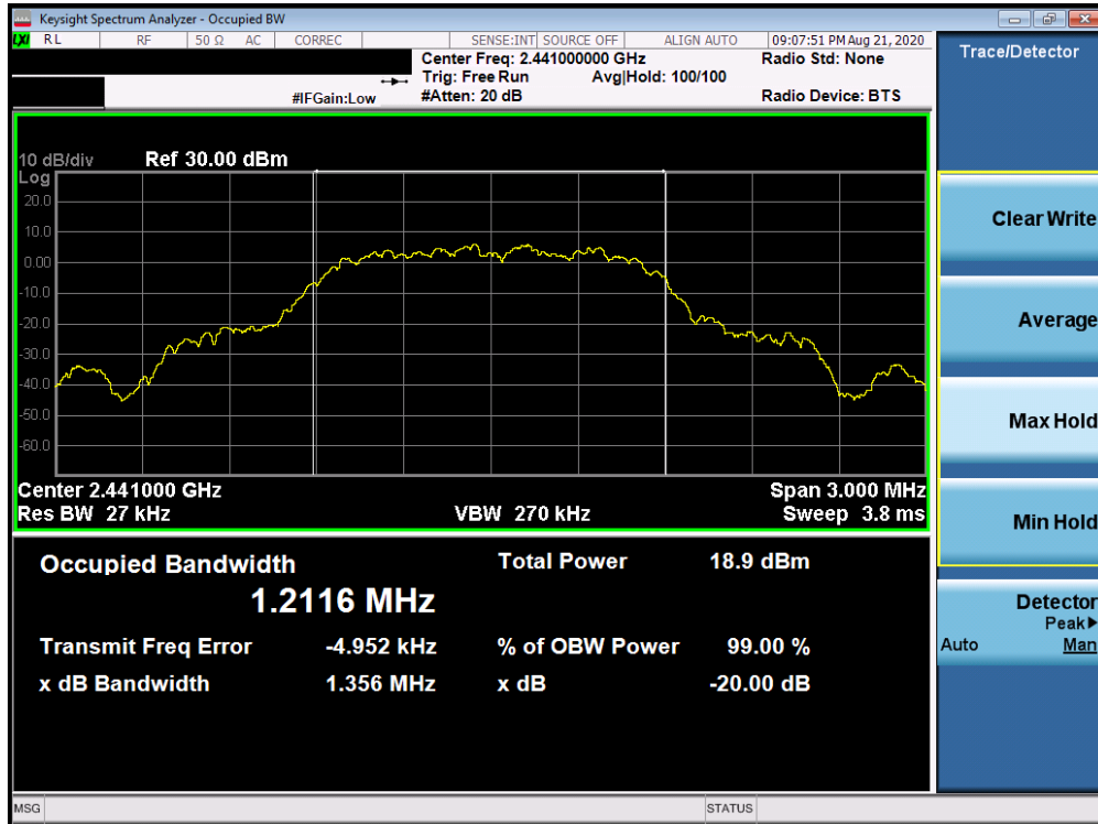
Plot 7-5. 20dB BW / 99% OBW Plot (Bluetooth, 8DPSK, iPA – Ch. 39)
