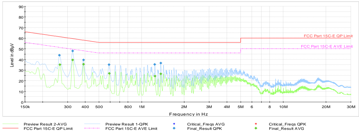
Plot 7-40. AC Line-Conducted Plot with GFSK iPA Ch.39 (N, with Laptop)
