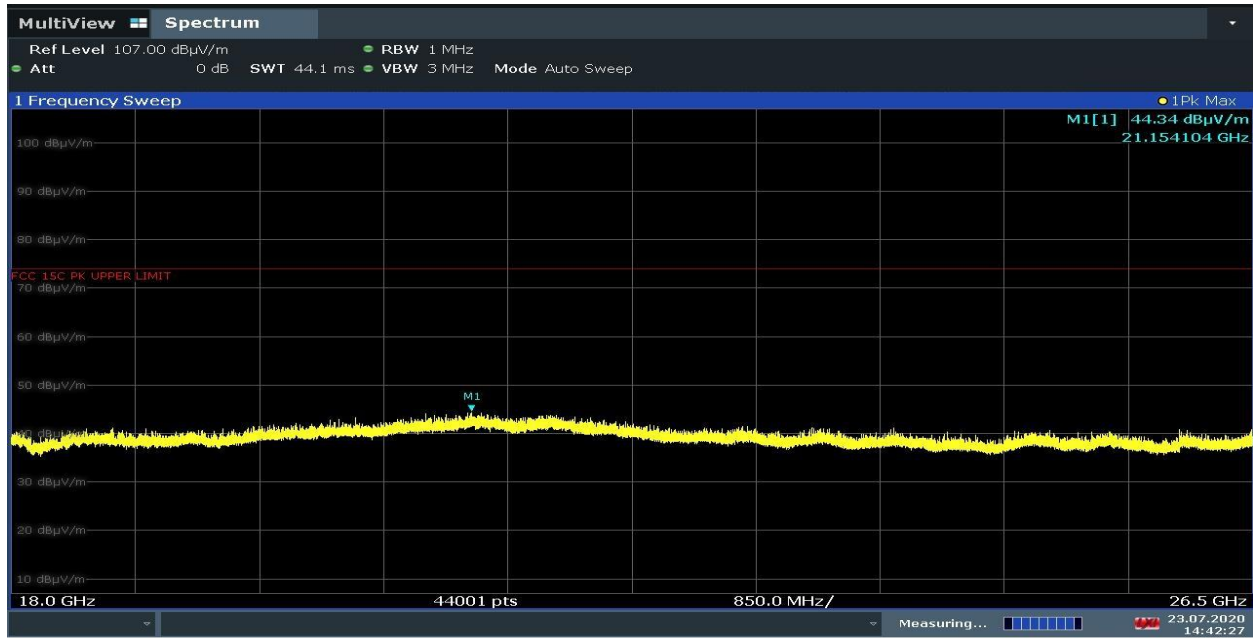
Plot 7-32. Radiated Spurious Emissions 18-26.5GHz (GFSK iPA – Ch.39, Pol. H)
