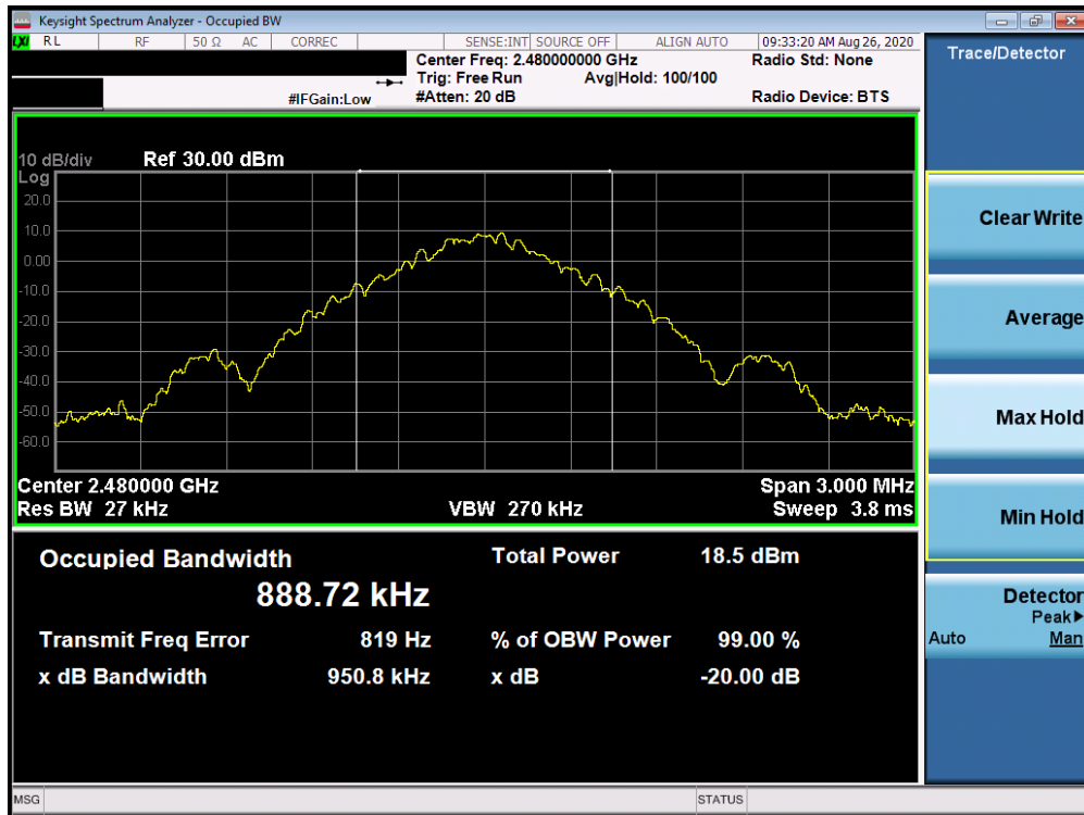
Plot 7-3. 20dB BW / 99% OBW Plot (Bluetooth, GFSK, iPA – Ch. 78)
