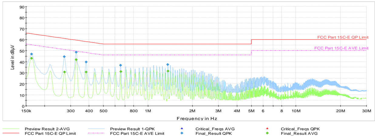
Plot 7-39. AC Line-Conducted Plot with GFSK iPA Ch.39 (L1, with Laptop)
