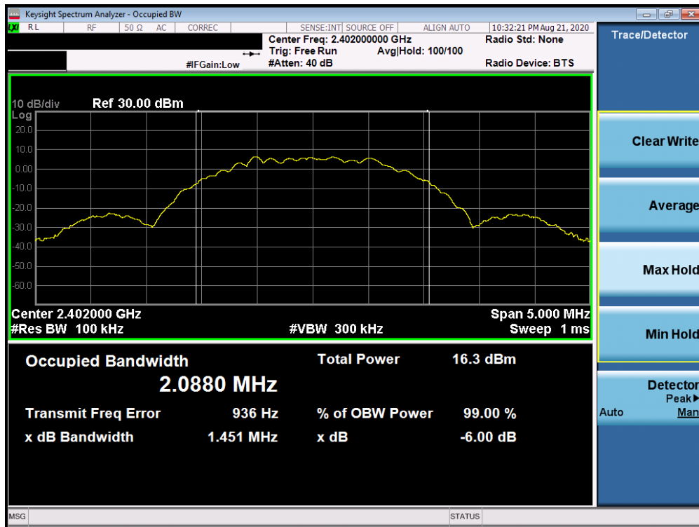
Plot 7-4. 6dB BW / 99% OBW Plot (Bluetooth (LE), 2Mbps, iPA – Ch. 0)
