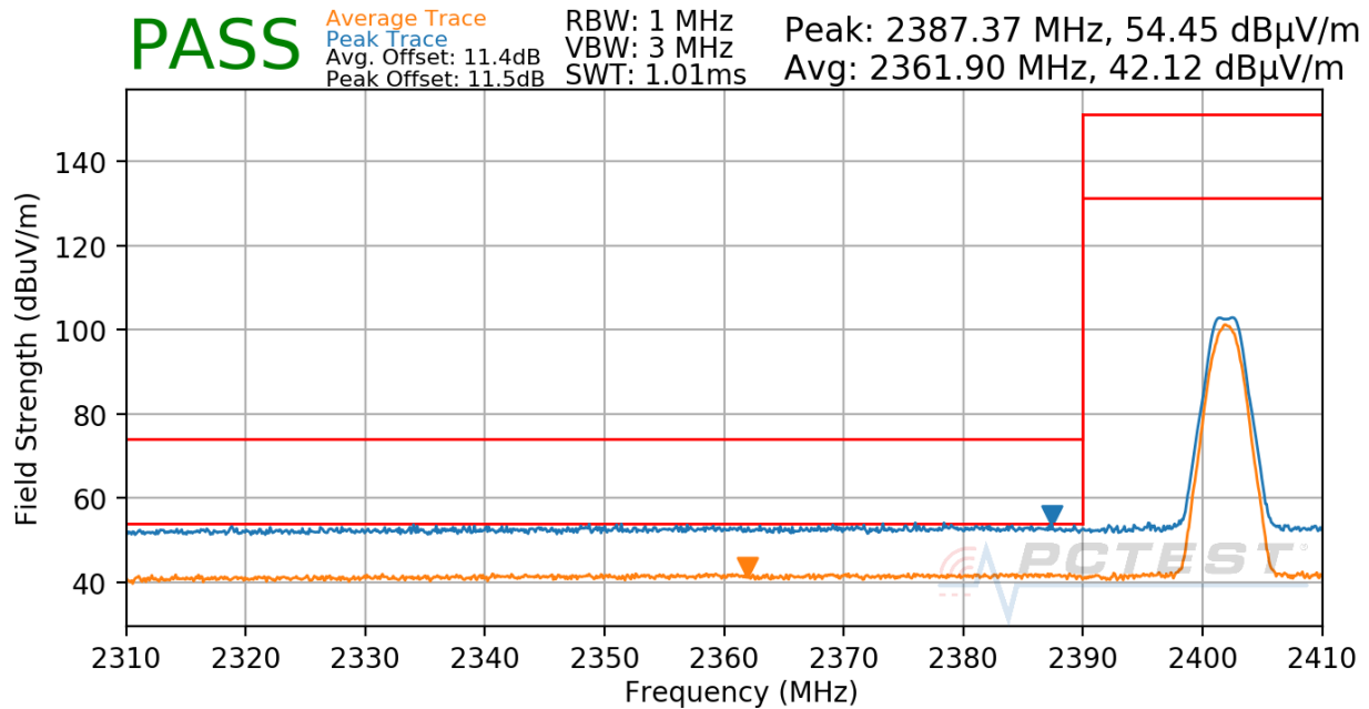
Plot 7-29. Radiated Restricted Lower Band Edge Measurement
