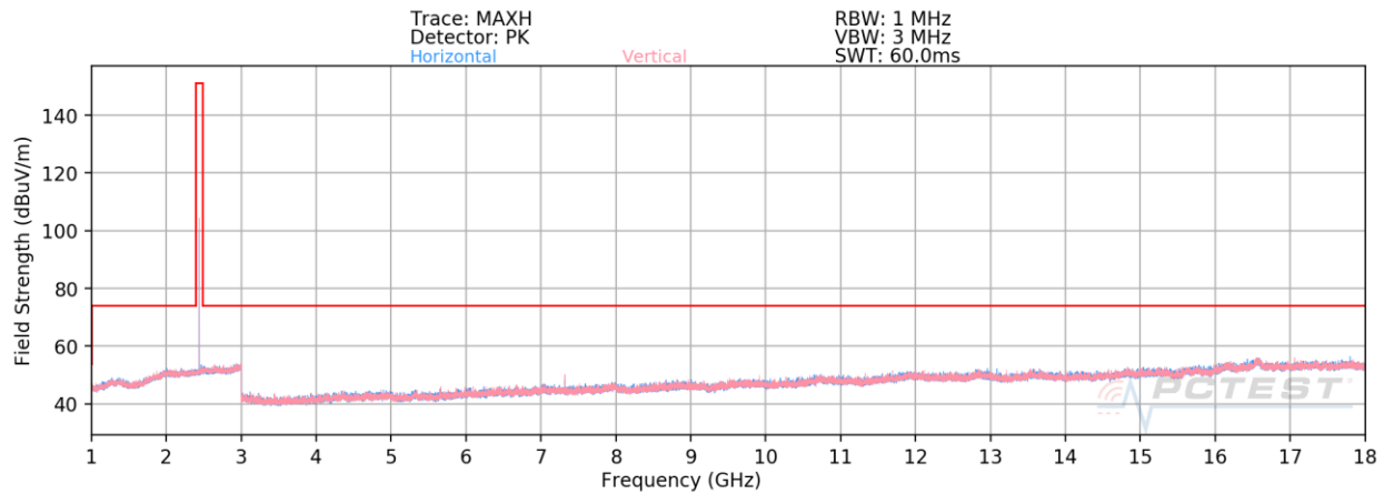
Plot 7-24. Radiated Spurious Emissions 1-18GHz (1Mbps, iPA – Ch. 19)
