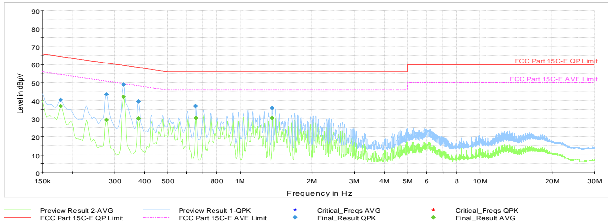
Plot 7-33. AC Line Conducted Plot with Bluetooth LE (L1 – 1Mbps, iPA, Ch.19, with Laptop)
