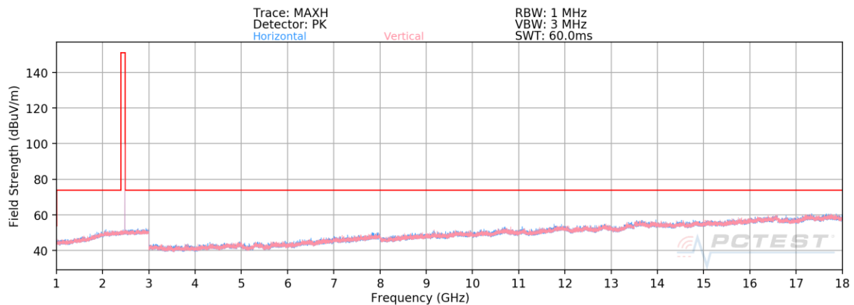
Plot 7-25. Radiated Spurious Emissions 1-18GHz (1Mbps, iPA – Ch. 39)
