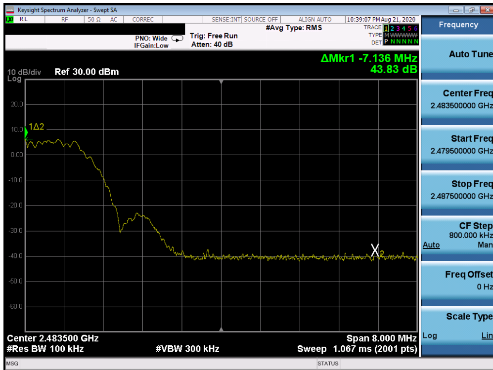
Plot 7-16. Band Edge Plot (Bluetooth (LE), 2Mbps, iPA - Ch. 39)
