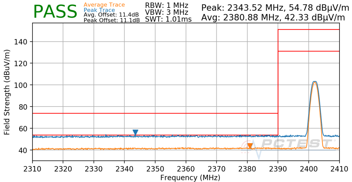
Plot 7-28. Radiated Restricted Lower Band Edge Measurement
