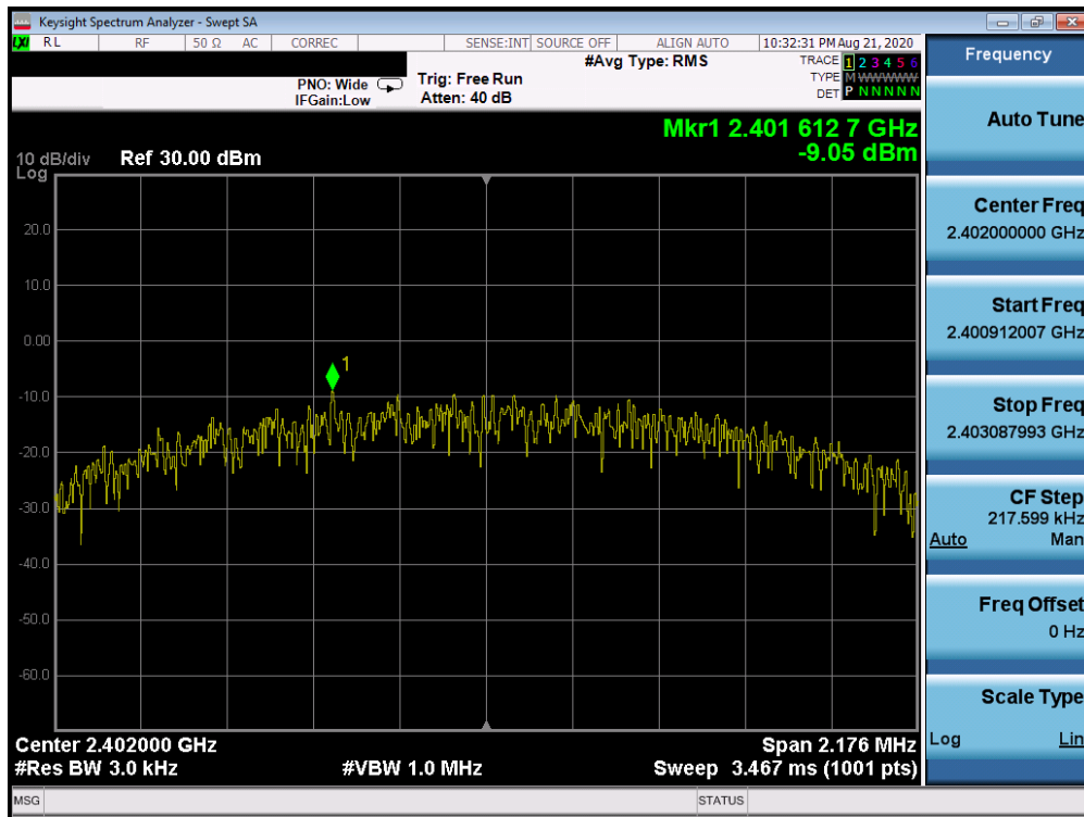
Plot 7-10. Power Spectral Density Plot (Bluetooth (LE), 2Mbps, iPA – Ch. 0)
