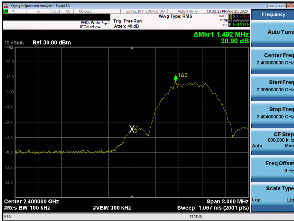
Plot 7-15. Band Edge Plot (Bluetooth (LE), 2Mbps, iPA - Ch. 0)
