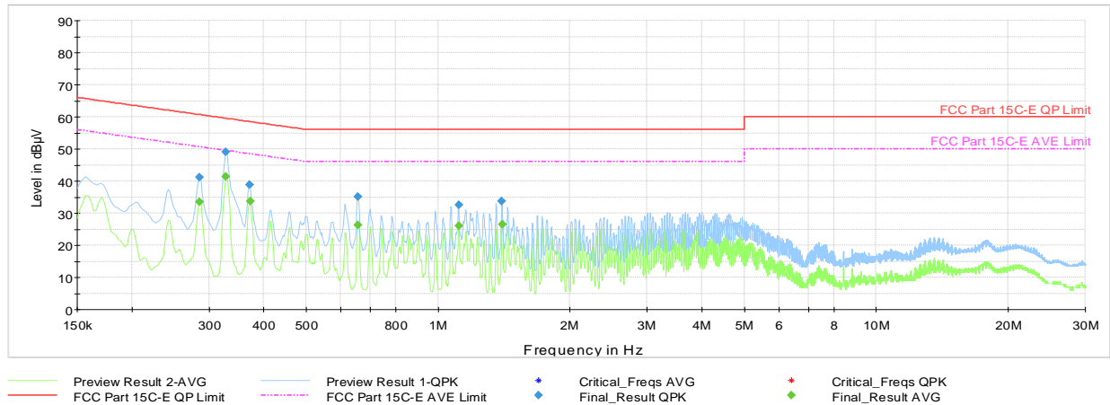
Plot 7-34. AC Line Conducted Plot with Bluetooth LE (N – 1Mbps, iPA, Ch.19, with Laptop)
