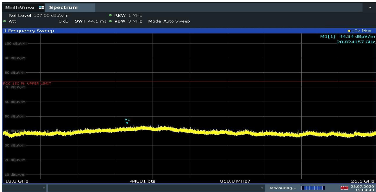
Plot 7-27. Radiated Spurious Plot Above 18GHz (1Mbps, iPA – Ch.19, Pol. V)
