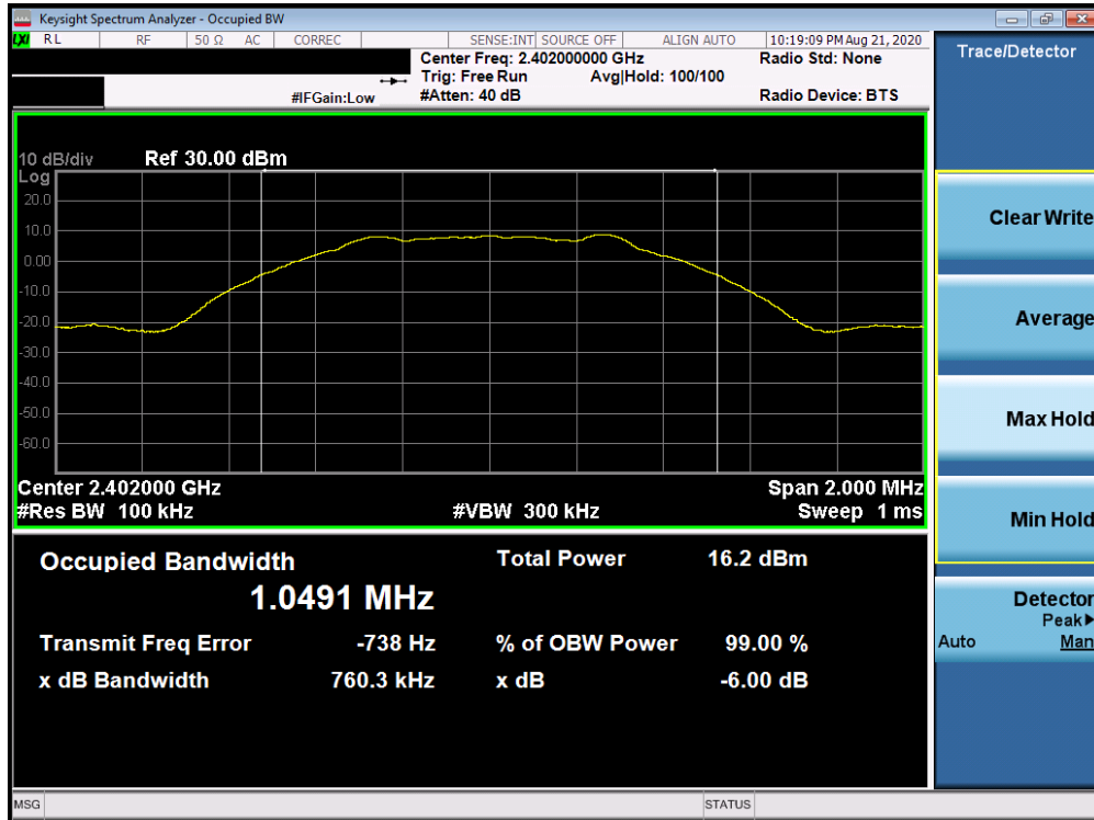
Plot 7-1. 6dB BW / 99% OBW Plot (Bluetooth (LE), 1Mbps, iPA – Ch. 0)
