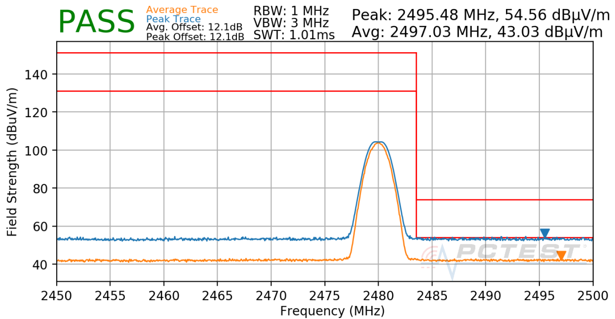
Plot 7-30. Radiated Restricted Upper Band Edge Measurement
