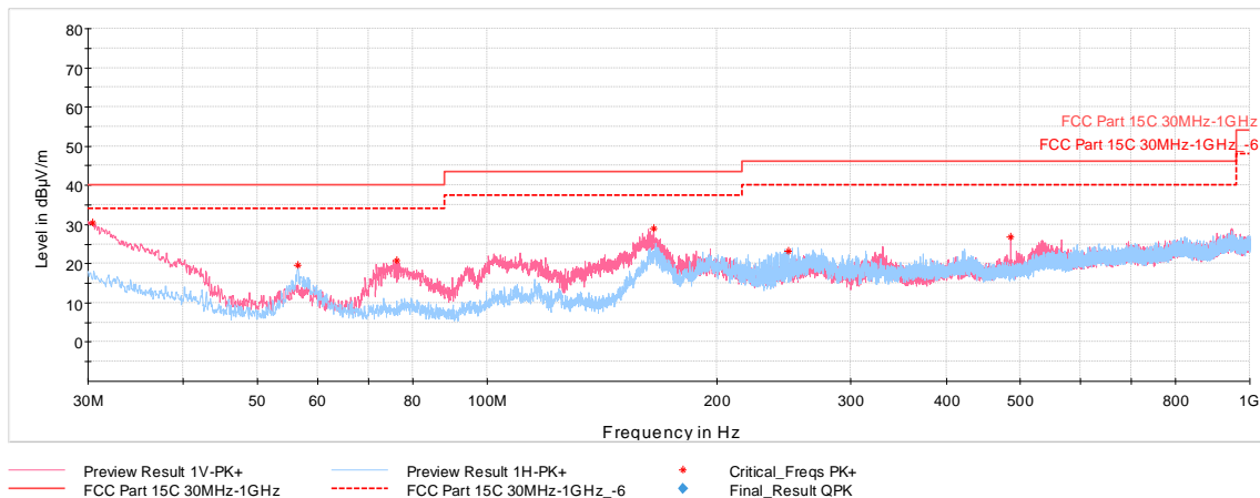
Plot 7-32. Radiated Spurious Emissions 30MHz-1GHz (1Mbps, iPA – Ch.19, with Laptop)
