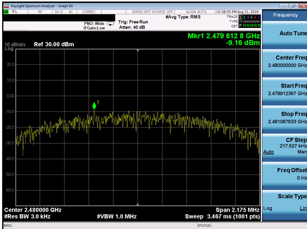
Plot 7-12. Power Spectral Density Plot (Bluetooth (LE), 2Mbps, iPA – Ch. 39)
