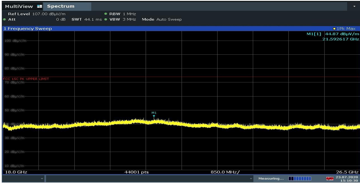
Plot 7-26. Radiated Spurious Plot Above 18GHz (1Mbps, iPA – Ch.19, Pol. H)
