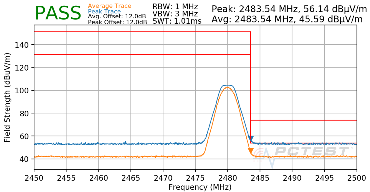
Plot 7-31. Radiated Restricted Upper Band Edge Measurement
