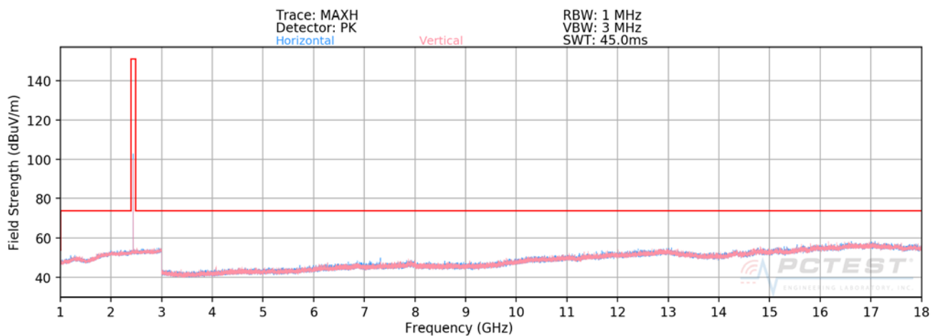
Plot 7-30. Radiated Spurious Plot Above 1GHz (1Mbps, ePA – Ch. 19)
