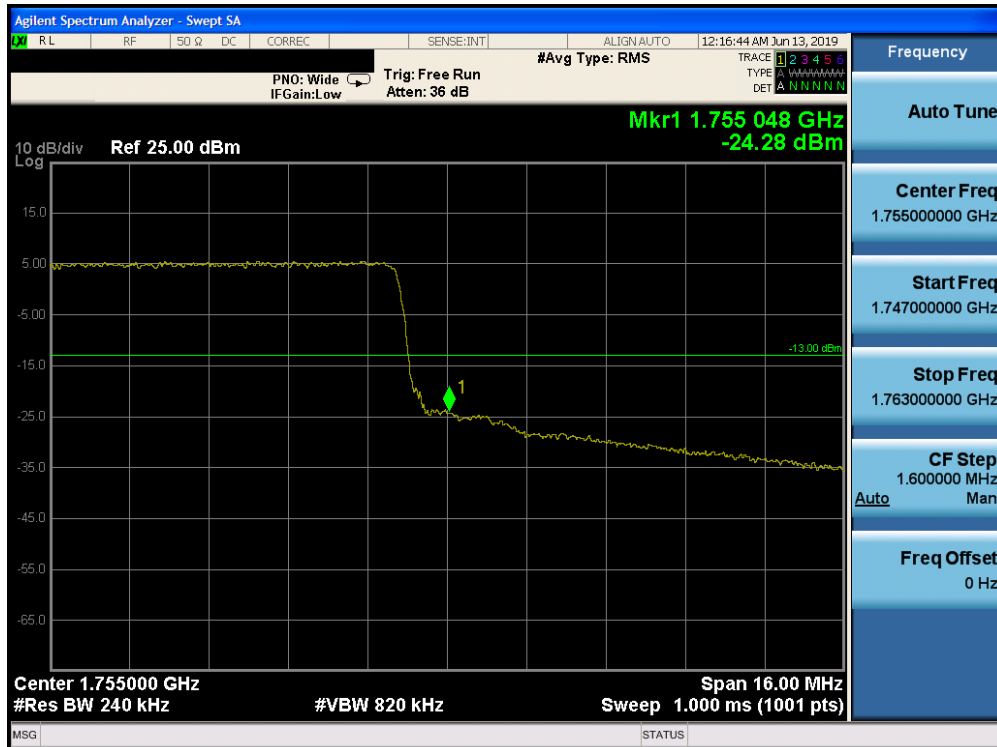
Plot 7-202. Upper Band Edge Plot (Band 4 - 20.0MHz QPSK - Full RB Configuration)
