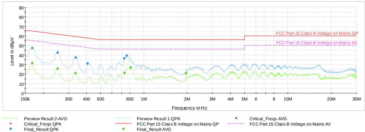
Plot 7-40. Line Conducted Plot with Bluetooth HDR (N- 4Mbps, ePA, Ch.38 with WCP + AC/DC Adapter)
