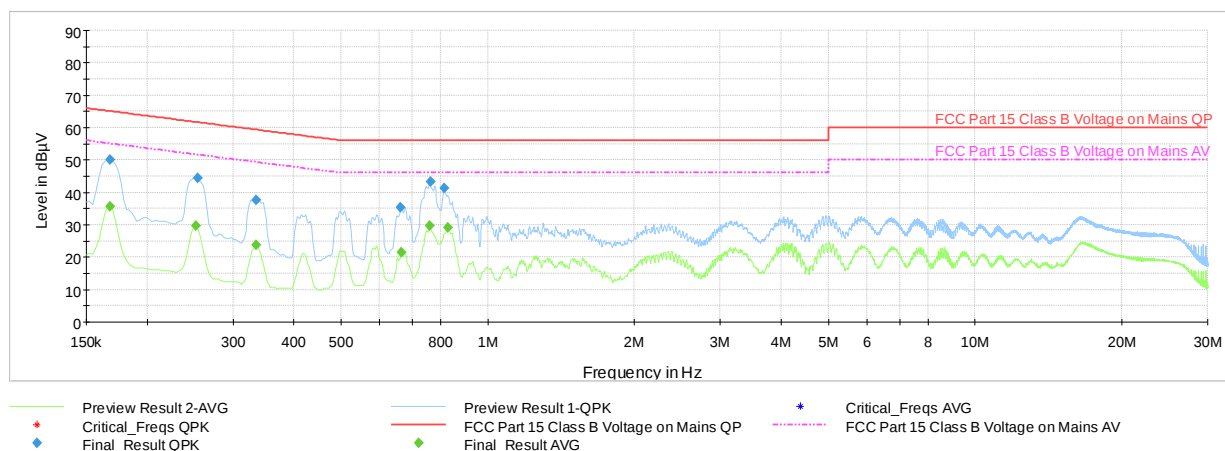
Plot 7-39. Line Conducted Plot with Bluetooth HDR (L1- 4Mbps, ePA, Ch.38 with WCP + AC/DC Adapter)
