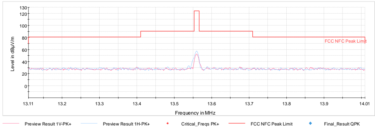
Plot 7-6. In Band Radiated Spurious Plot (CE A 848kbps)
