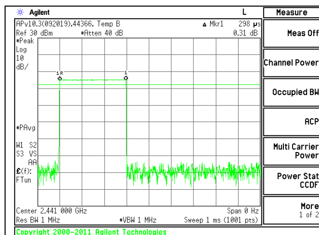
PULSE WIDTH – DM1
