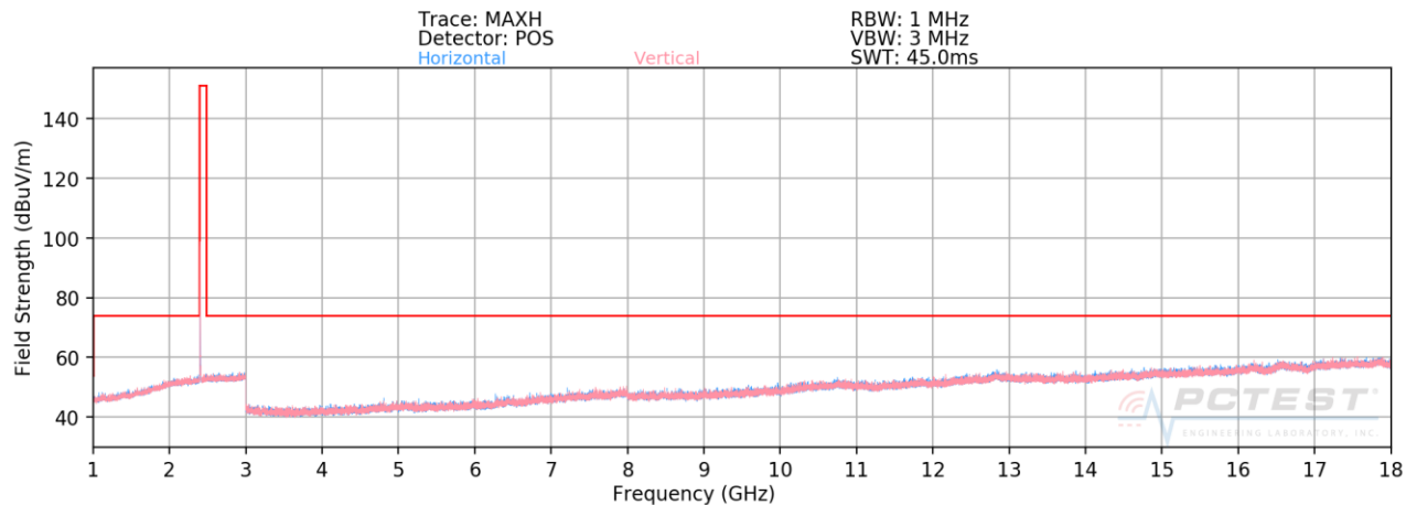
Plot 7-48. Radiated Spurious Plot ((HDR, ePA), 8Mbps – Ch. 1, Ant. Pol. H & V)
