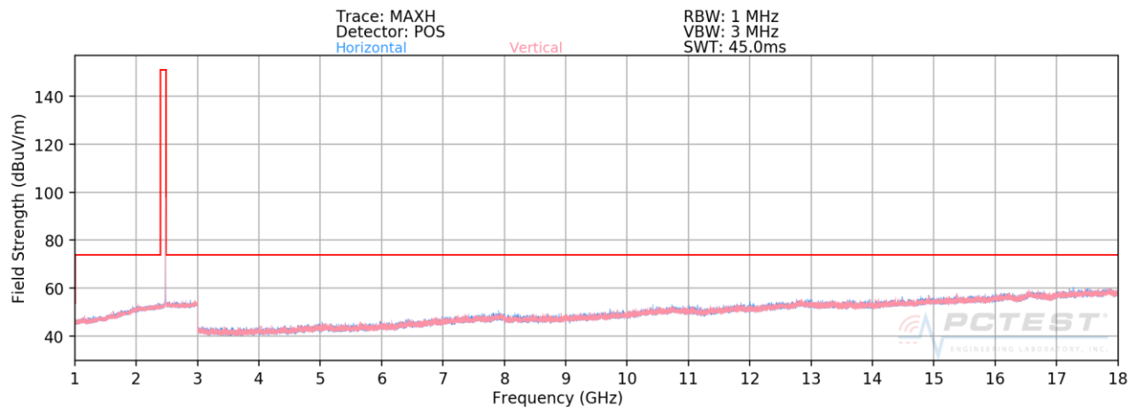
Plot 7-50. Radiated Spurious Plot ((HDR, ePA), 8Mbps – Ch. 75, Ant. Pol. H & V)
