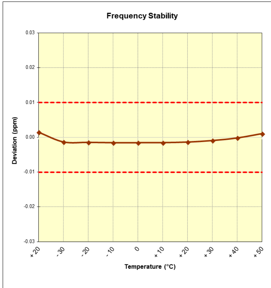
Figure 7-8. Frequency Stability Plot (Reader Ask 100% 1 out of 4)
