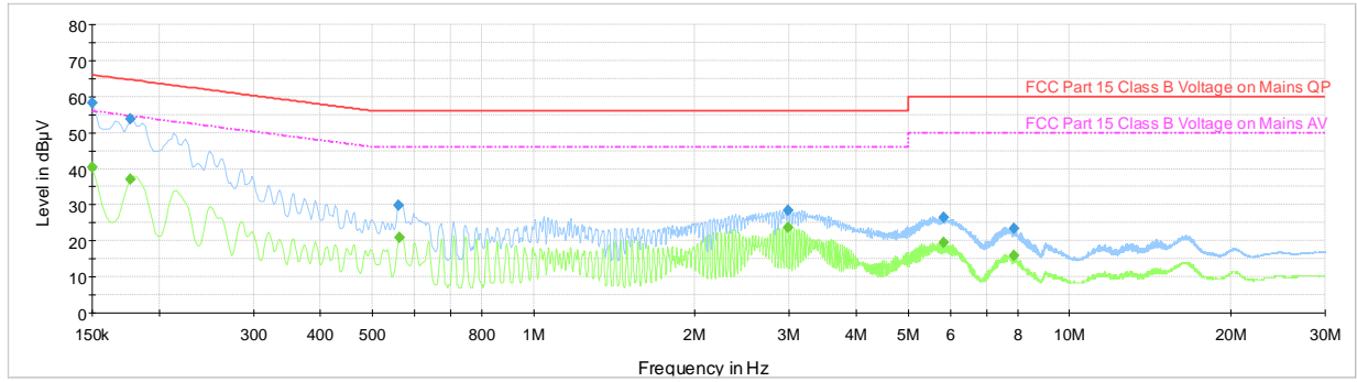
Plot 7-75. Line-Conducted Test Plot (L1)
