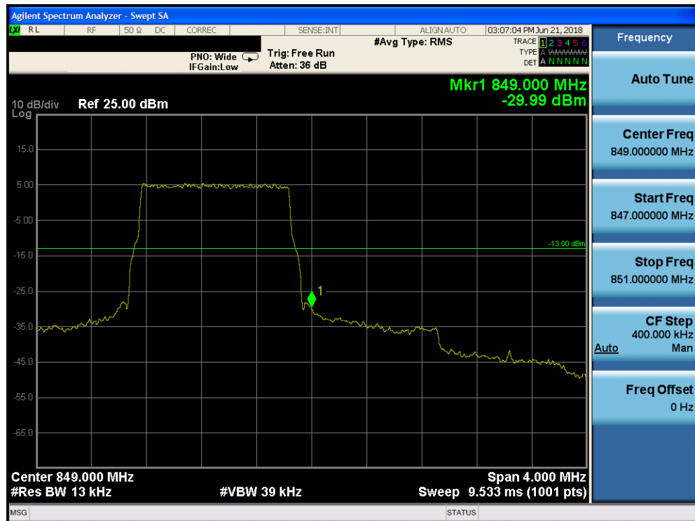
Plot 7-62. Upper Band Edge Plot (Band 26/5 - 1.4MHz QPSK - Full RB Configuration)
