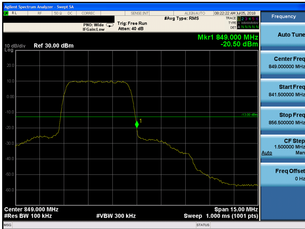
Plot 7-12. Band Edge Plot (Cellular WCDMA Mode - High Channel)
