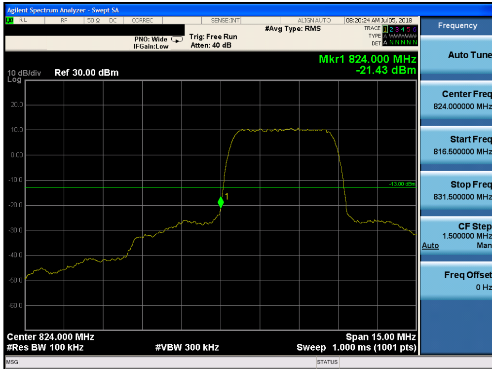
Plot 7-11. Band Edge Plot (Cellular WCDMA Mode - Low Channel)
