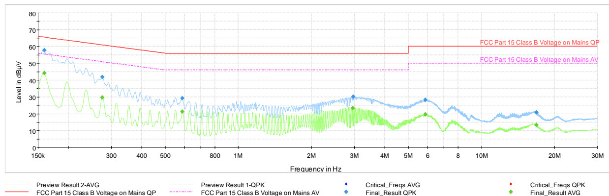
Plot 7-55. Line Conducted Plot with Bluetooth LE (L1)
