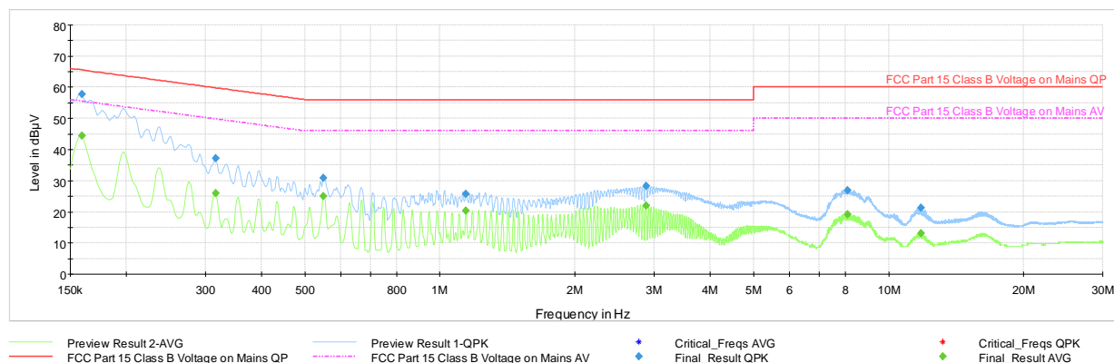
Plot 7-56. Line Conducted Plot with Bluetooth LE (N)
