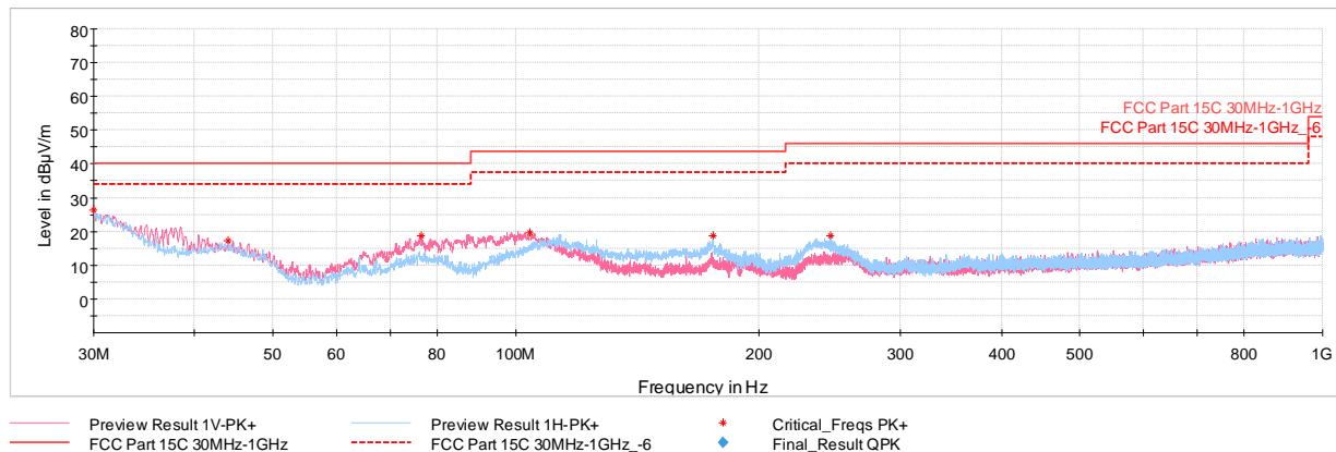
Plot 7-54. Radiated Spurious Plot below 1GHz (1Mbps, ePA, Pol. H & V, with WCP + AC/DC Adapter attached)
