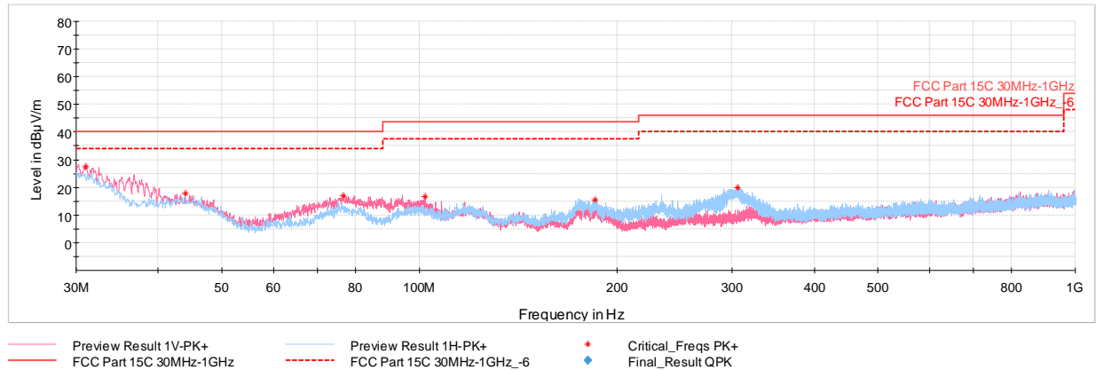
Plot 7-74. Radiated Spurious Plot below 1GHz (GFSK ePA, Pol. H & V, with WCP + Adapter attached)
