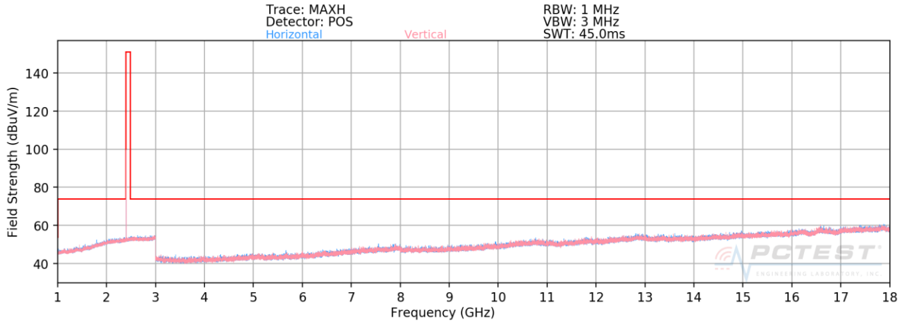
Plot 7-61. Radiated Spurious Plot above 1GHz (BT GFSK ePA – Ch. 0, Ant. Pol. H & V)
