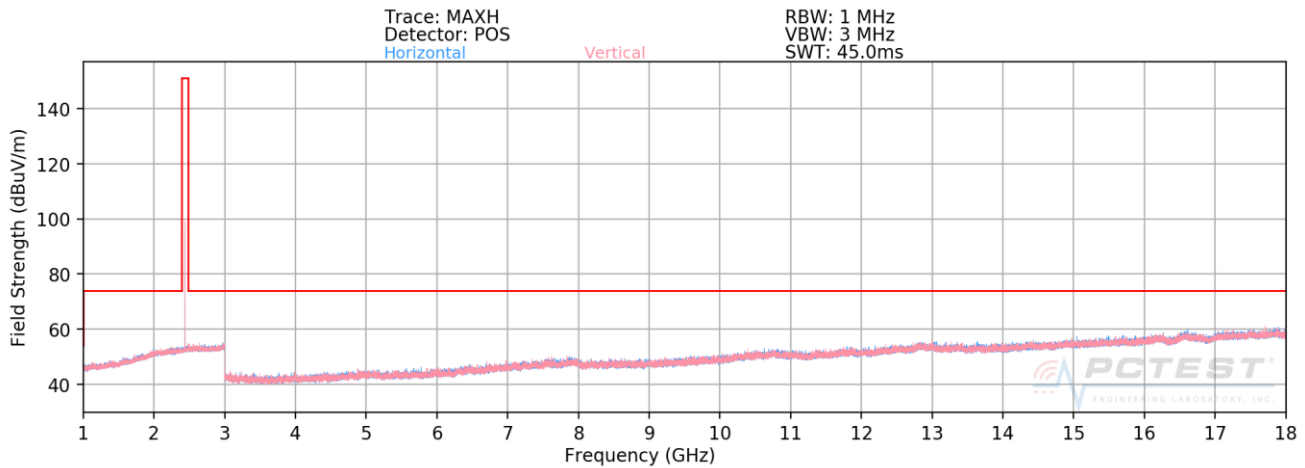
Plot 7-62. Radiated Spurious Plot above 1GHz (BT GFSK ePA – Ch. 39 Ant. Pol. H & V)
