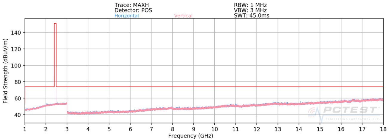
Plot 7-63. Radiated Spurious Plot above 1GHz (BT GFSK ePA – Ch. 78 Ant. Pol. H & V)
