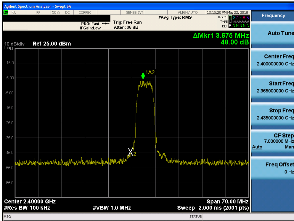
Plot 7-25. Band Edge Plot (Bluetooth (HDR, iPA), 8Mbps – Ch. 1)
