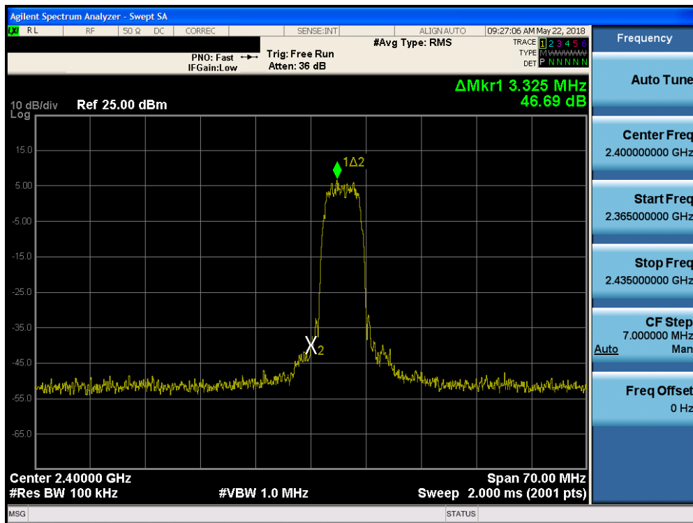
Plot 7-23. Band Edge Plot (Bluetooth (HDR, ePA), 8Mbps – Ch. 1)
