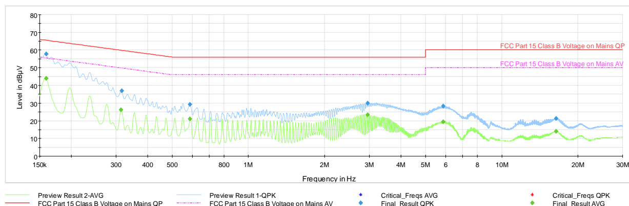
Plot 7-53. Line Conducted Plot with Bluetooth HDR (L1, with WCP + Laptop)
