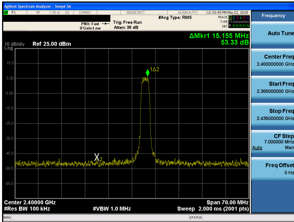
Plot 7-21. Band Edge Plot (Bluetooth (HDR, iPA), 4Mbps – Ch. 1)
