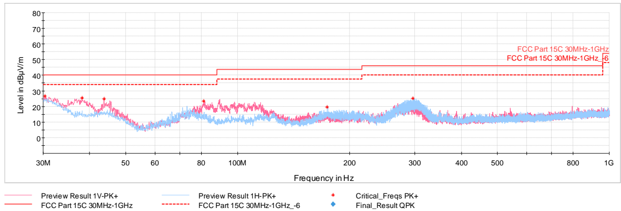
Plot 7-52. Radiated Spurious Plot below 1GHz (8Mbps, ePA, Pol. H & V, with WCP + Laptop)
