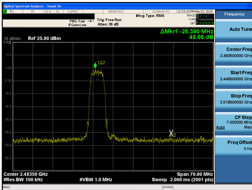
Plot 7-26. Band Edge Plot (Bluetooth (HDR, iPA), 8Mbps – Ch. 75)
