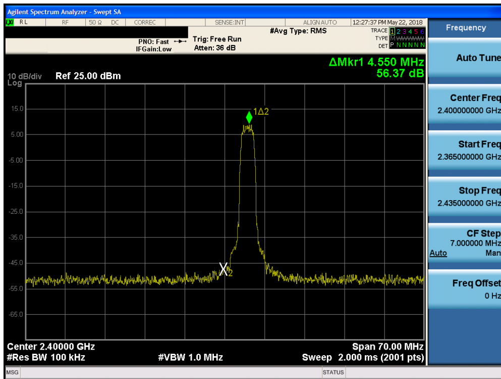
Plot 7-19. Band Edge Plot (Bluetooth (HDR, ePA), 4Mbps – Ch. 1)
