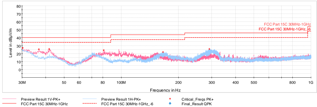
Plot 7-51. Radiated Spurious Plot below 1GHz (4Mbps, ePA, Pol. H & V, with WCP + Laptop attached)
