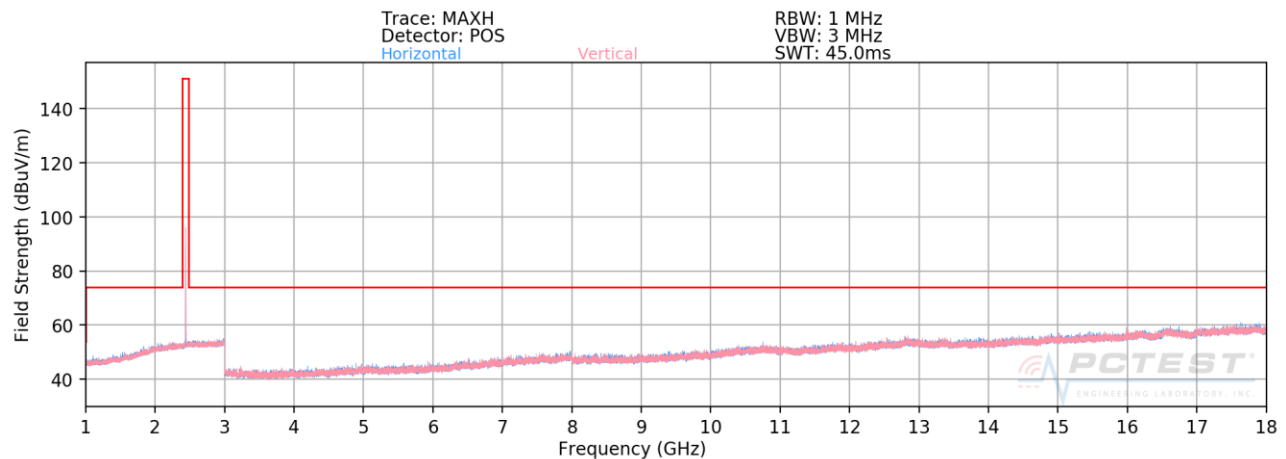
Plot 7-43. Radiated Spurious Plot above 1GHz (8Mbps, ePA – Ch.38, Ant. Pol. H & V)
