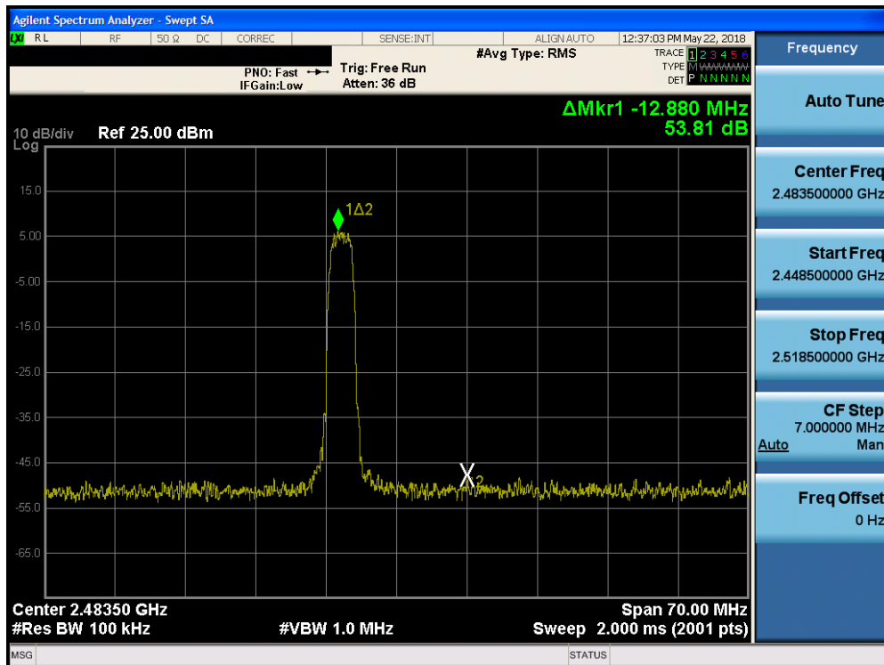
Plot 7-22. Band Edge Plot (Bluetooth (HDR, iPA), 4Mbps – Ch. 75)
