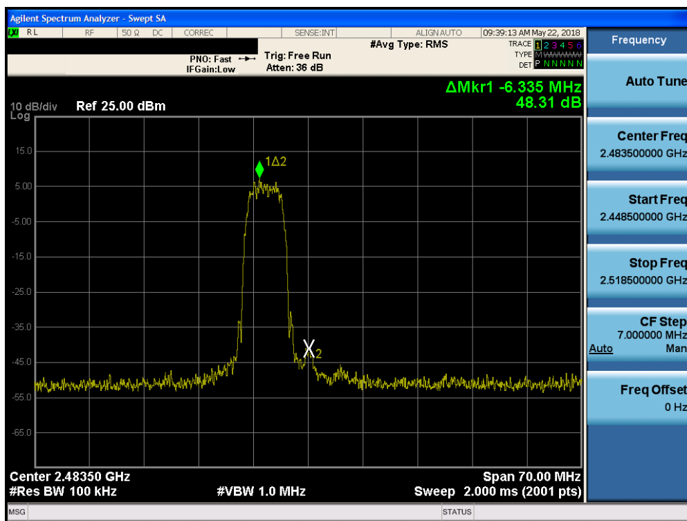
Plot 7-24. Band Edge Plot (Bluetooth (HDR, ePA), 8Mbps – Ch. 75)
