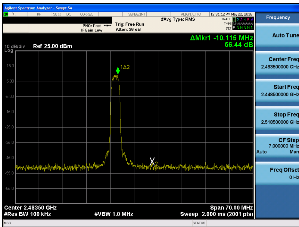
Plot 7-20. Band Edge Plot (Bluetooth (HDR, ePA), 4Mbps – Ch. 75)
