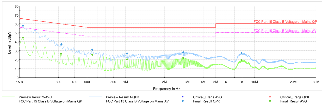
Plot 7-54. Line Conducted Plot with Bluetooth HDR (N, with WCP + Laptop)
