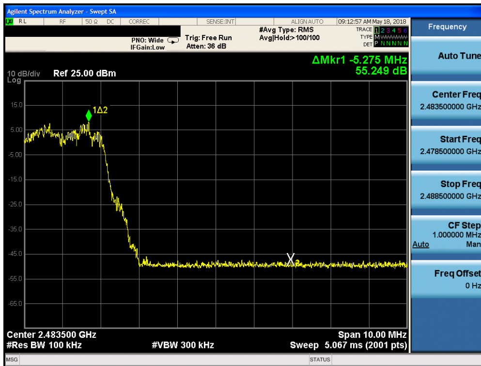
Plot 7-40. Band Edge Plot (Bluetooth with Hopping Enabled, 8DPSK, iPA)
