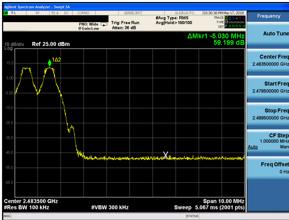
Plot 7-32. Band Edge Plot (Bluetooth with Hopping Enabled, GFSK, iPA)
