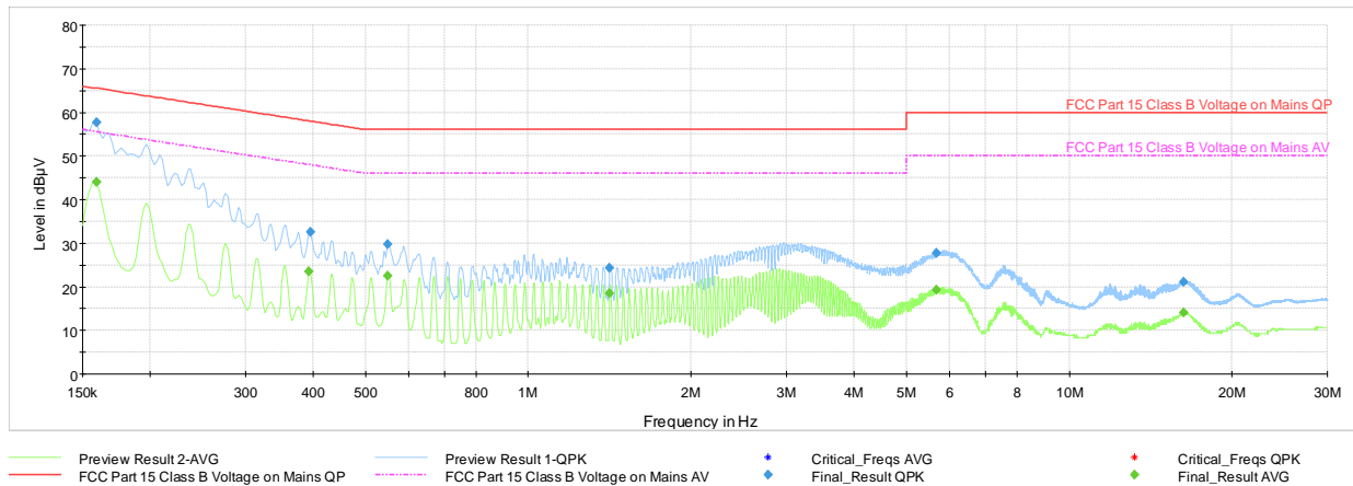
Plot 7-75. Line-Conducted Test Plot (L1)
