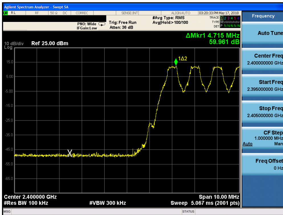
Plot 7-31. Band Edge Plot (Bluetooth with Hopping Enabled, GFSK, iPA)
