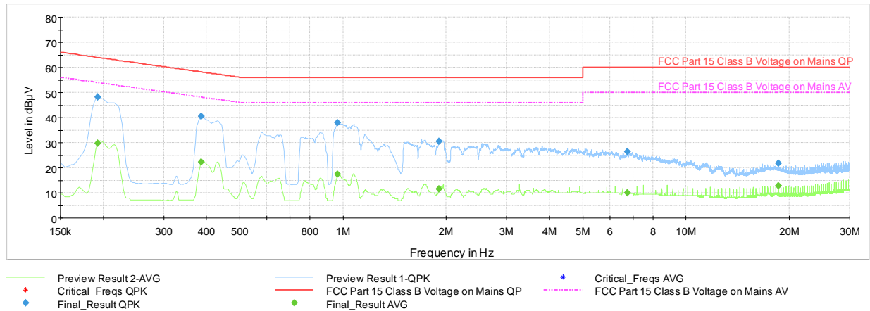
Plot 7-47. Line Conducted Plot with 802.11b (L1 with WCP + AC/DC Adapter attached)
