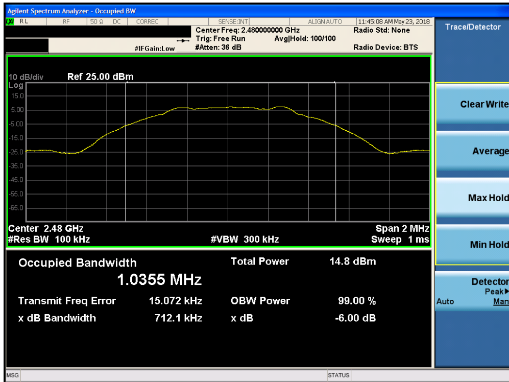
Plot 7-6. 6dB Bandwidth Plot (Bluetooth (LE), 1Mbps, iPA – Ch. 39)
