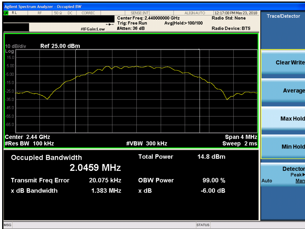
Plot 7-8. 6dB Bandwidth Plot (Bluetooth (LE), 2Mbps, ePA – Ch. 19)
