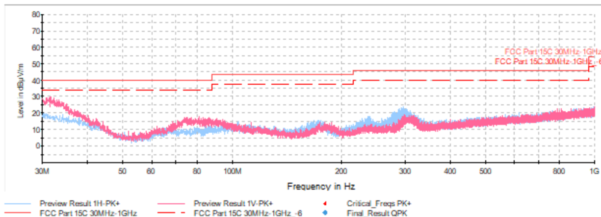
Plot 7-5. Radiated Spurious Plot 30MHz – 1GHz (CE A 848kdps, Pol. H & V, with WCP + AC/DC Adapter attached)
