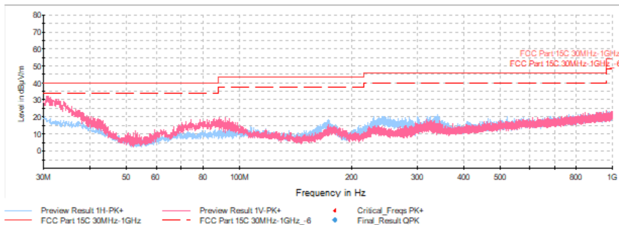
Plot 7-6. Radiated Spurious Plot 30MHz – 1GHz (Reader 100 Ask 1 out of 4, Pol. H & V, with WCP + AC/DC Adapter attached)
