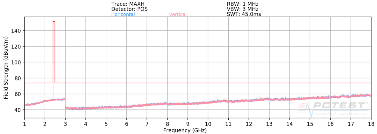
Plot 7-39. Radiated Spurious Plot above 1GHz (4Mbps, ePA – Ch.1, Ant. Pol. H & V)
