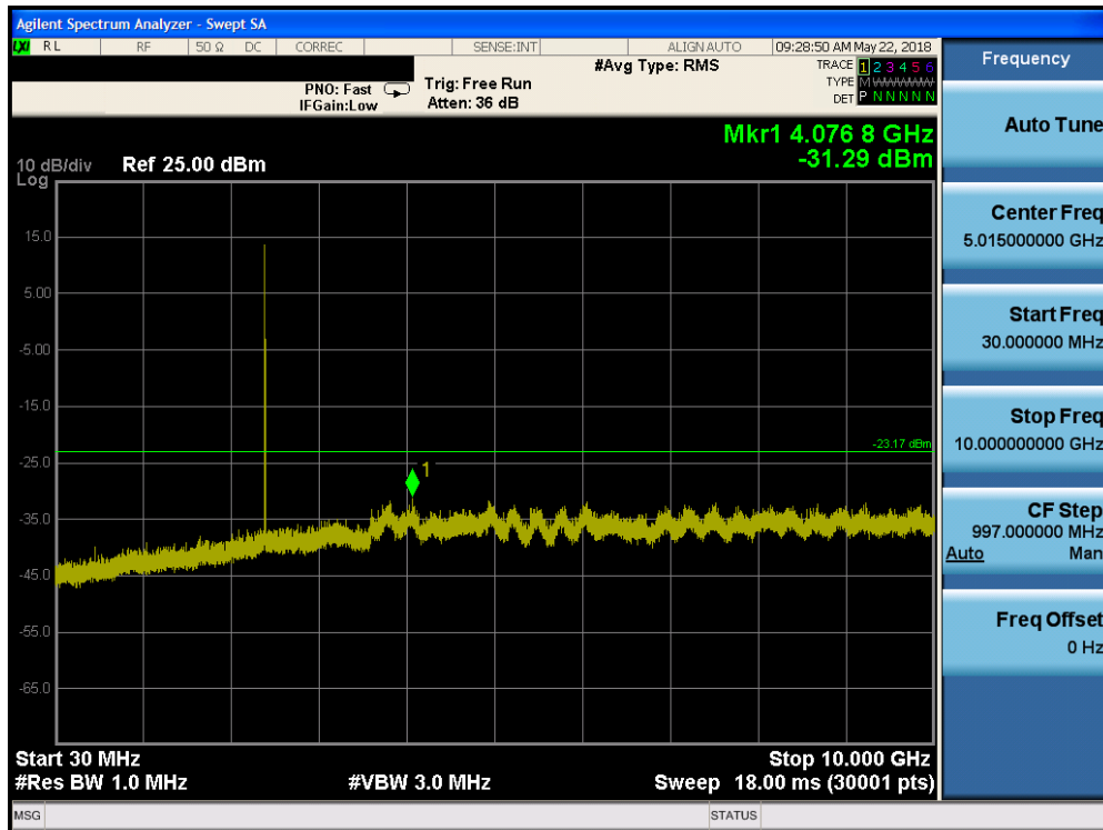
Plot 7-33. Conducted Spurious Plot (Bluetooth (HDR), 8Mbps, ePA – Ch. 1)
