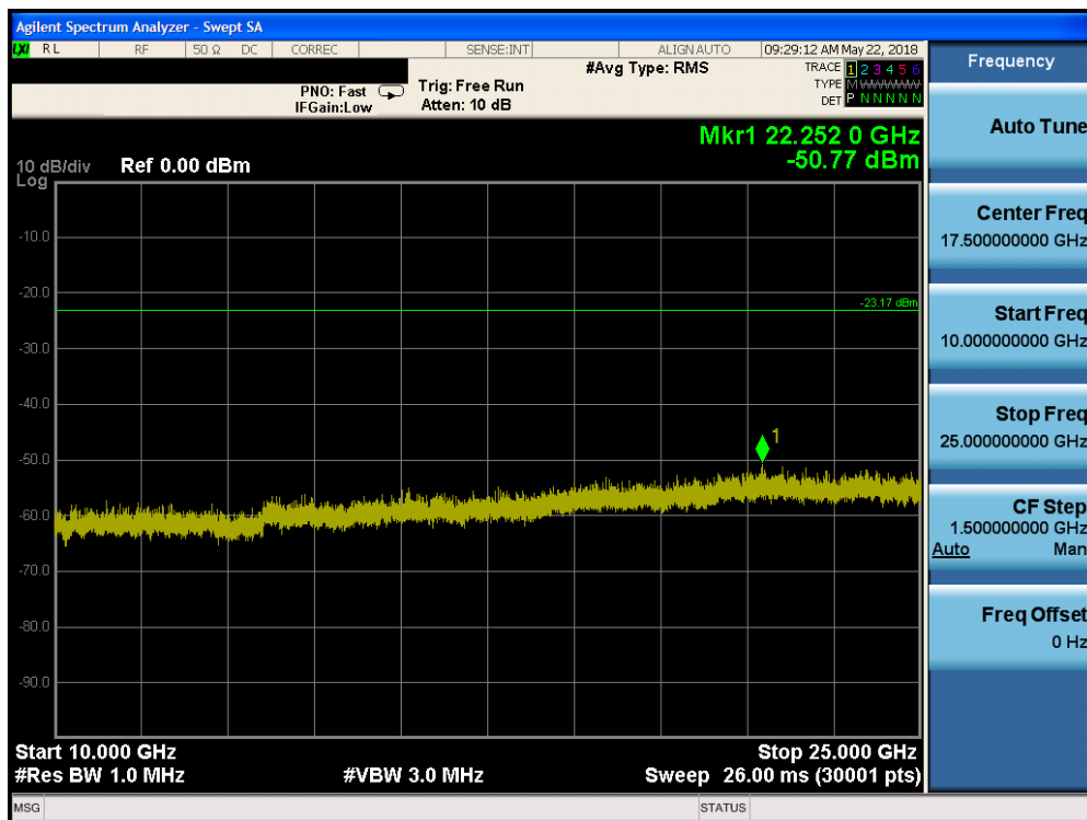
Plot 7-34. Conducted Spurious Plot (Bluetooth (HDR), 8Mbps, ePA – Ch. 1)
