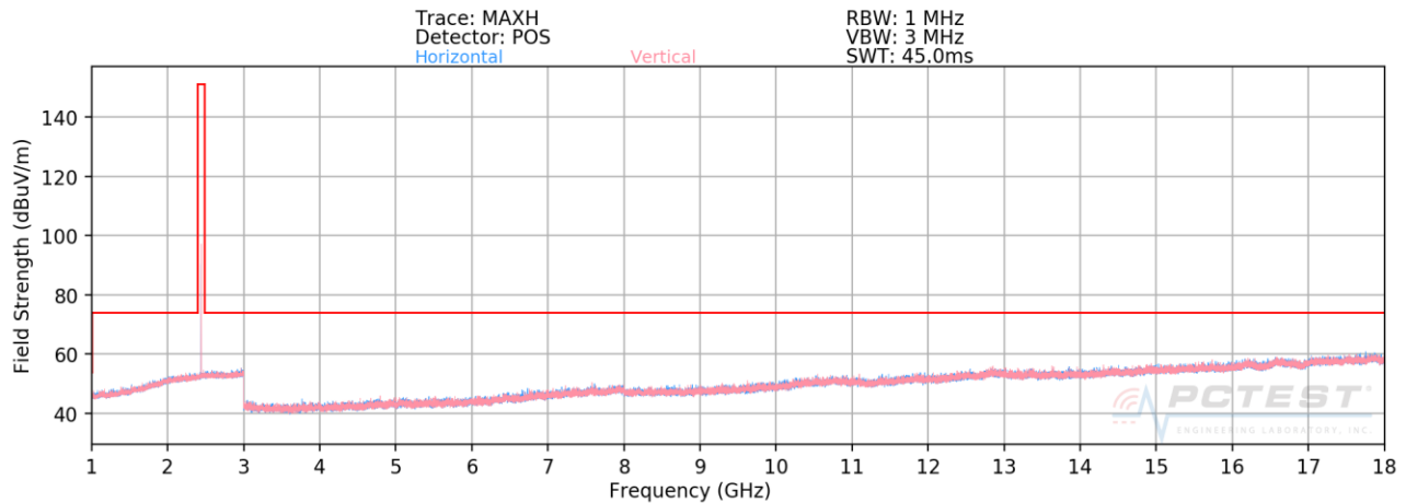
Plot 7-40. Radiated Spurious Plot above 1GHz (4Mbps, ePA – Ch.38, Ant. Pol. H & V)
