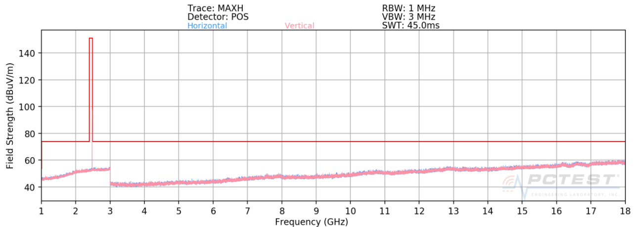
Plot 7-41. Radiated Spurious Plot above 1GHz (4Mbps, ePA – Ch.75, Ant. Pol. H & V)
