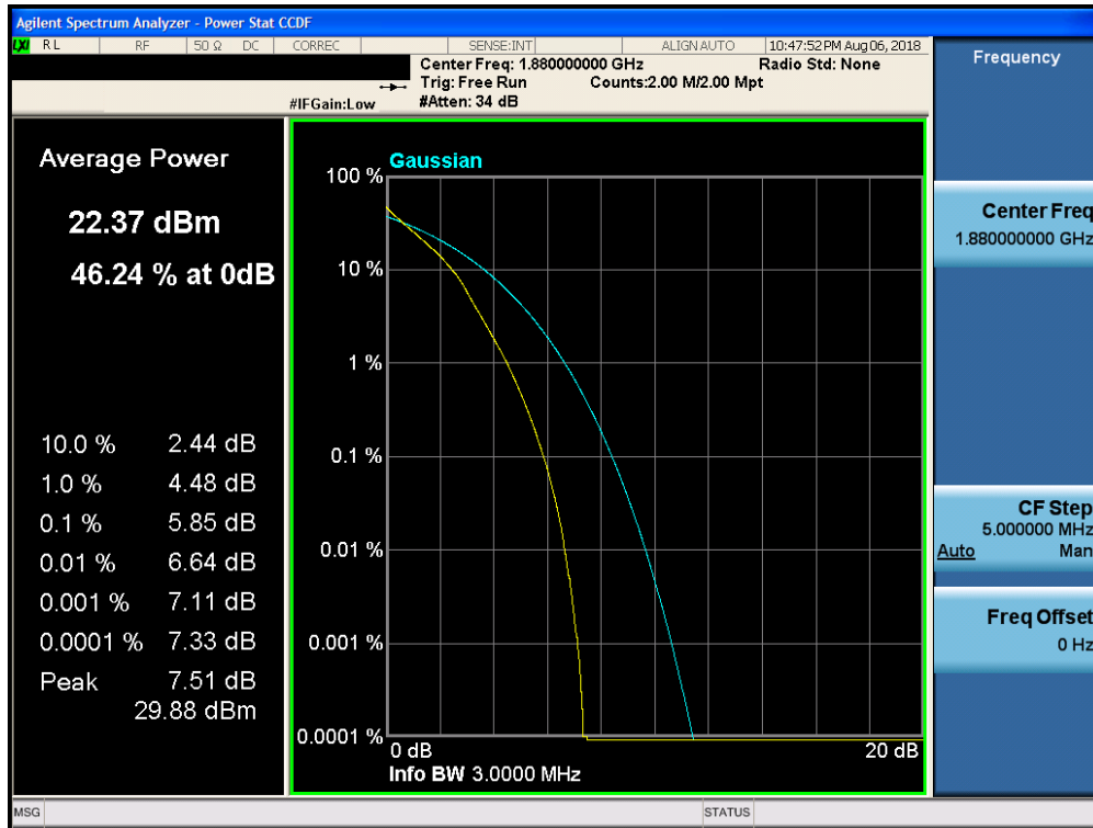
Plot 7-304. PAR Plot (Band 2 - 3.0MHz QPSK - Full RB Configuration)
