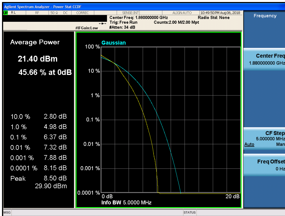
Plot 7-307. PAR Plot (Band 2 - 5.0MHz 16-QAM - Full RB Configuration)
