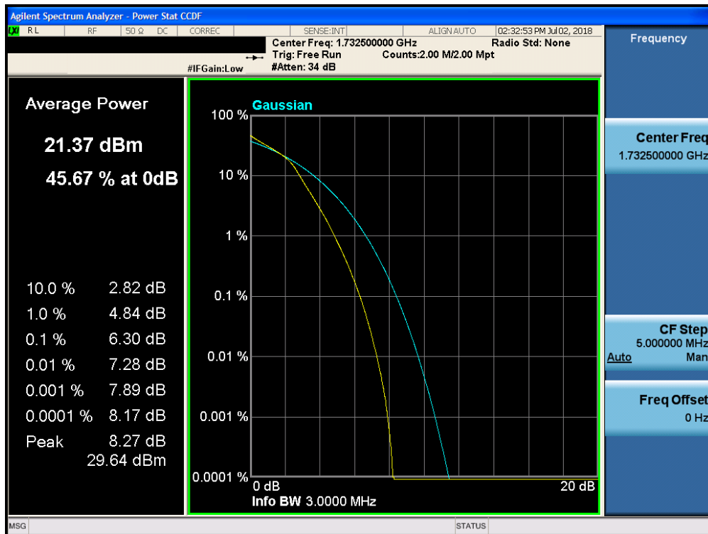
Plot 7-281. PAR Plot (Band 4 - 3.0MHz 16-QAM - Full RB Configuration)
