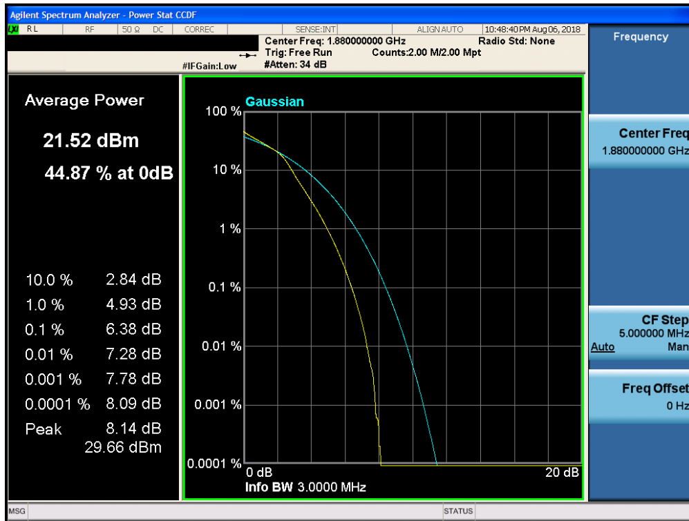
Plot 7-305. PAR Plot (Band 2 - 3.0MHz 16-QAM - Full RB Configuration)
