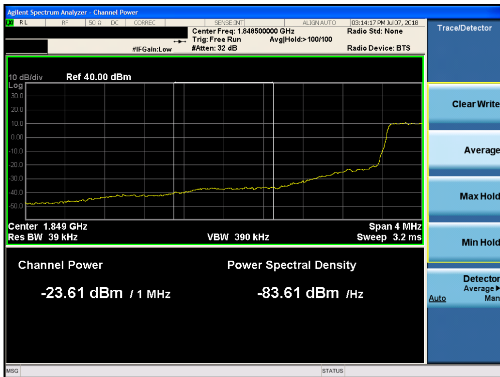
Plot 7-247. Lower Extended Band Edge Plot (Band 2 - 1.4MHz QPSK - Full RB Configuration)
