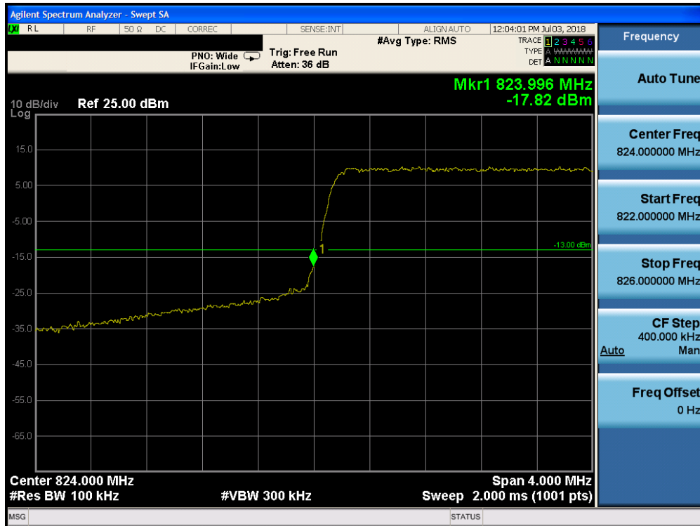
Plot 7-192. Lower Band Edge Plot (Band 5 - 3.0MHz QPSK - Full RB Configuration)
